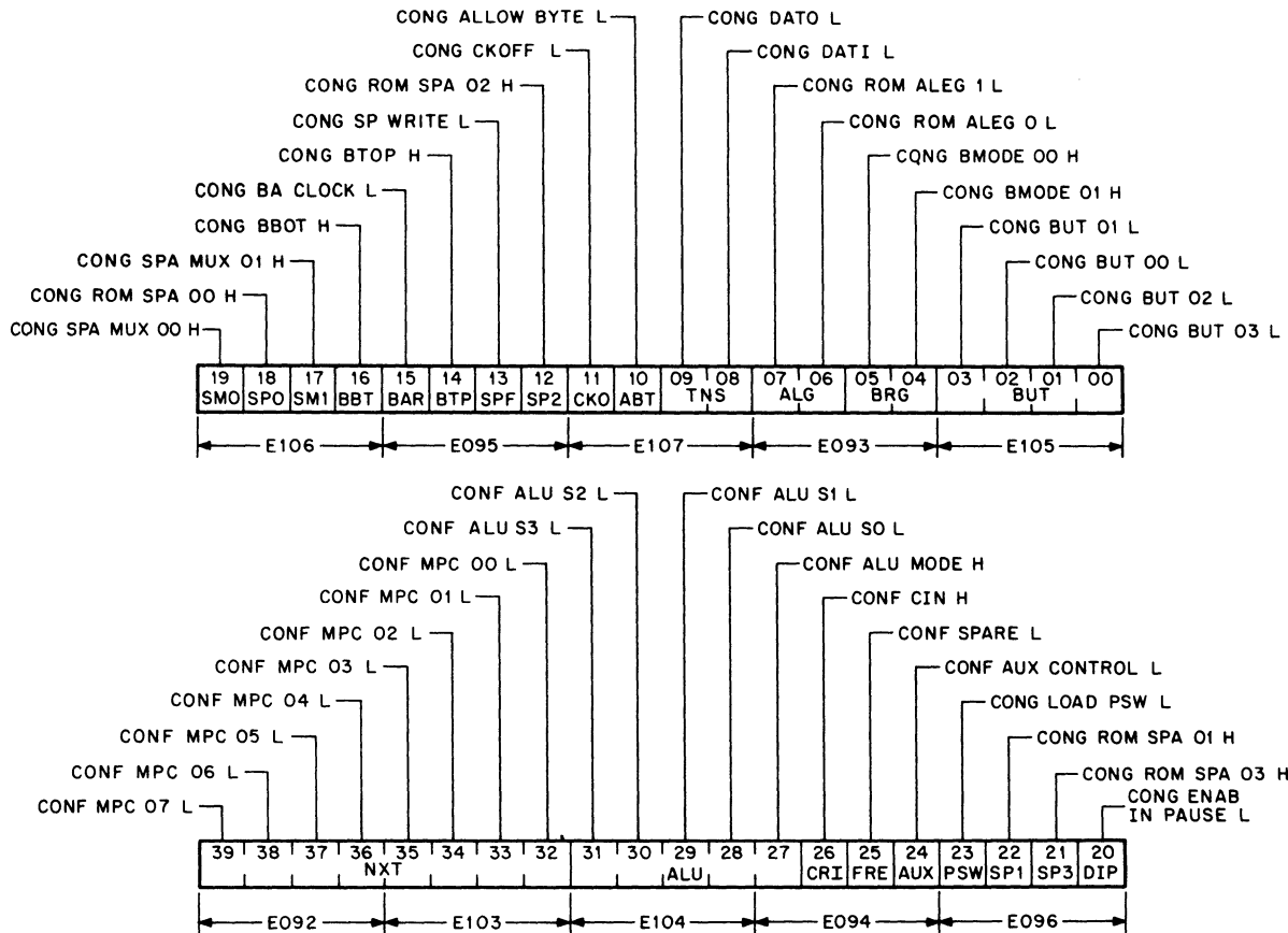
Figure 9-1 Control Store Word Bit and Field Format
