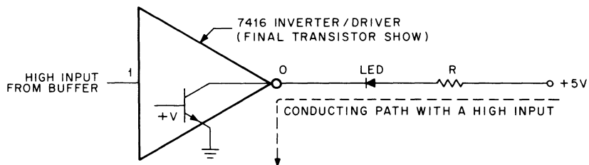
Figure 7-5 LED Driver Circuit
