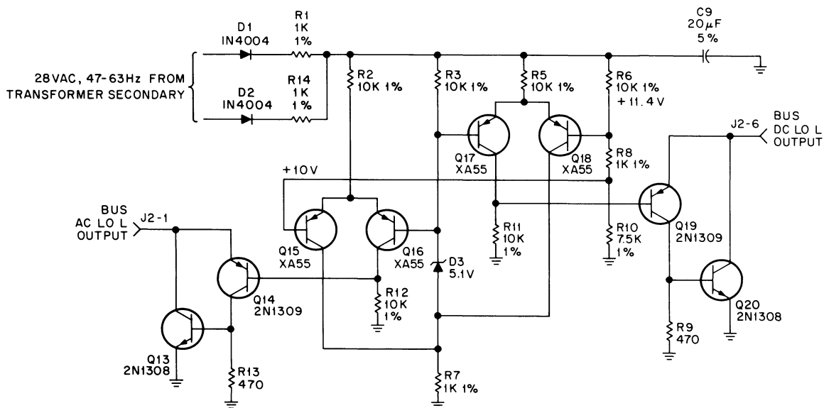
Figure 3-16 BUS AC LO and BUS DC LO Circuits
