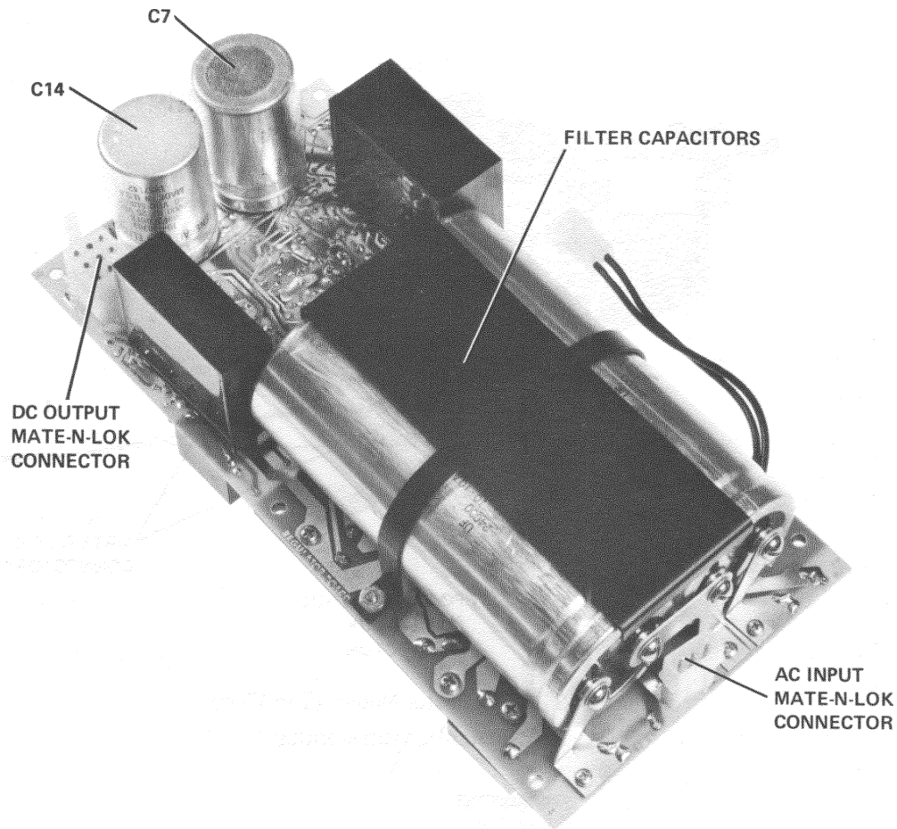
Figure 14-2 Power Supply Assembly (with DC Regulator Module Removed)
