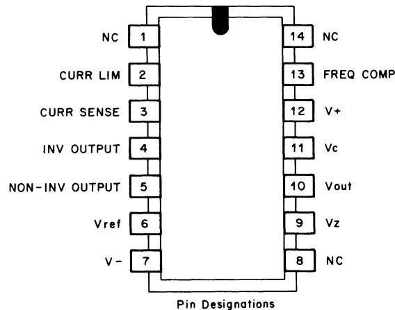
Figure 3-22 Voltage Regulator (E1) Equivalent Circuit and Package Configuration
