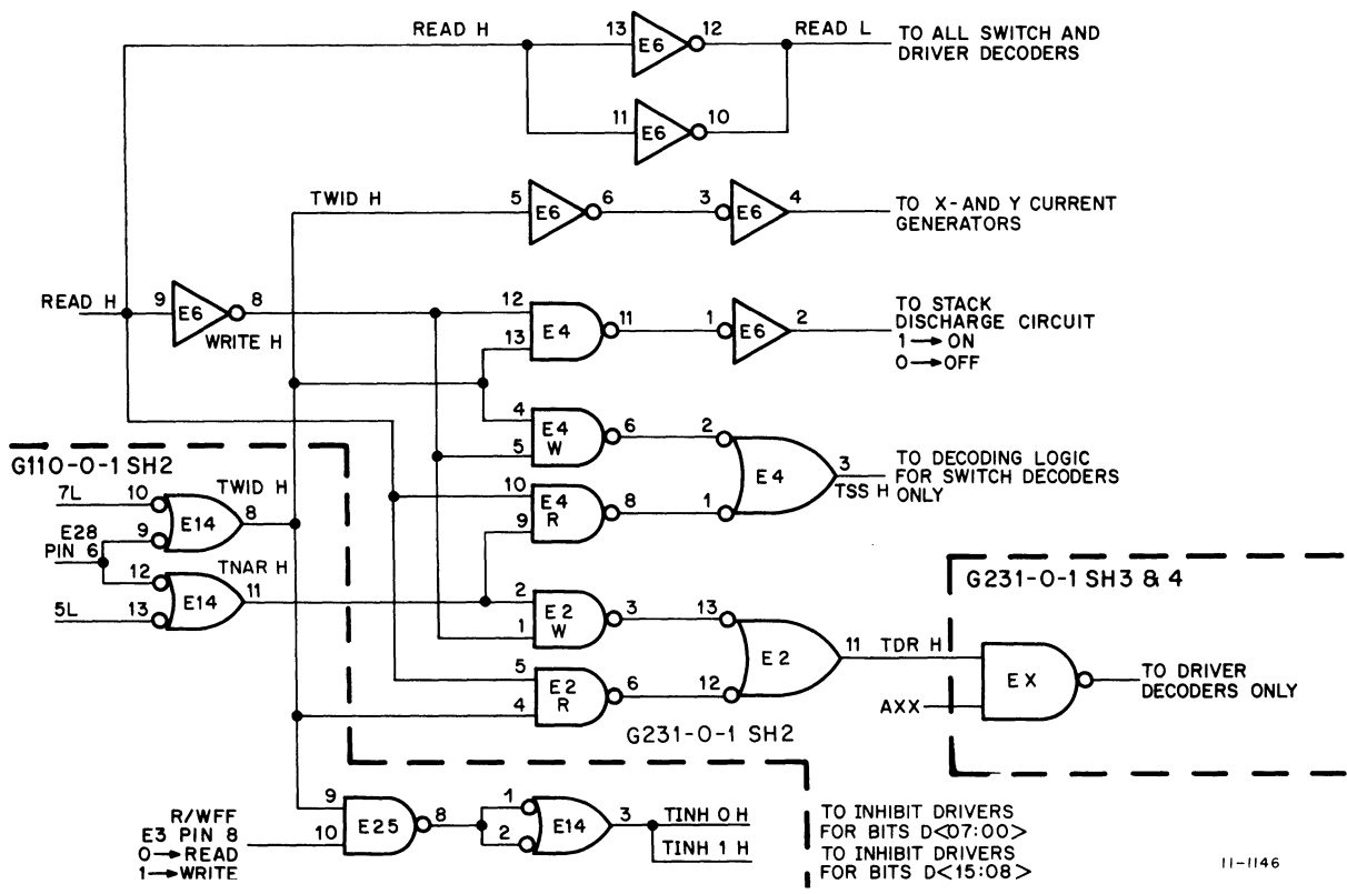
Figure 12-21 TWID H and TNAR H Control Logic
