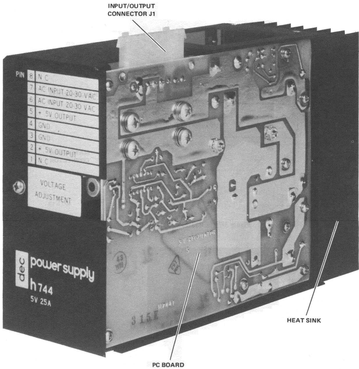
Figure 3-6 +5 V Regulator, 3/4 Bottom View
