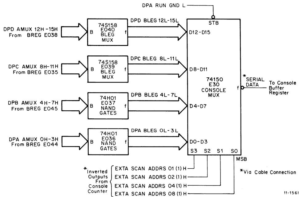
Figure 8-13 Console Multiplexer Block Diagram
