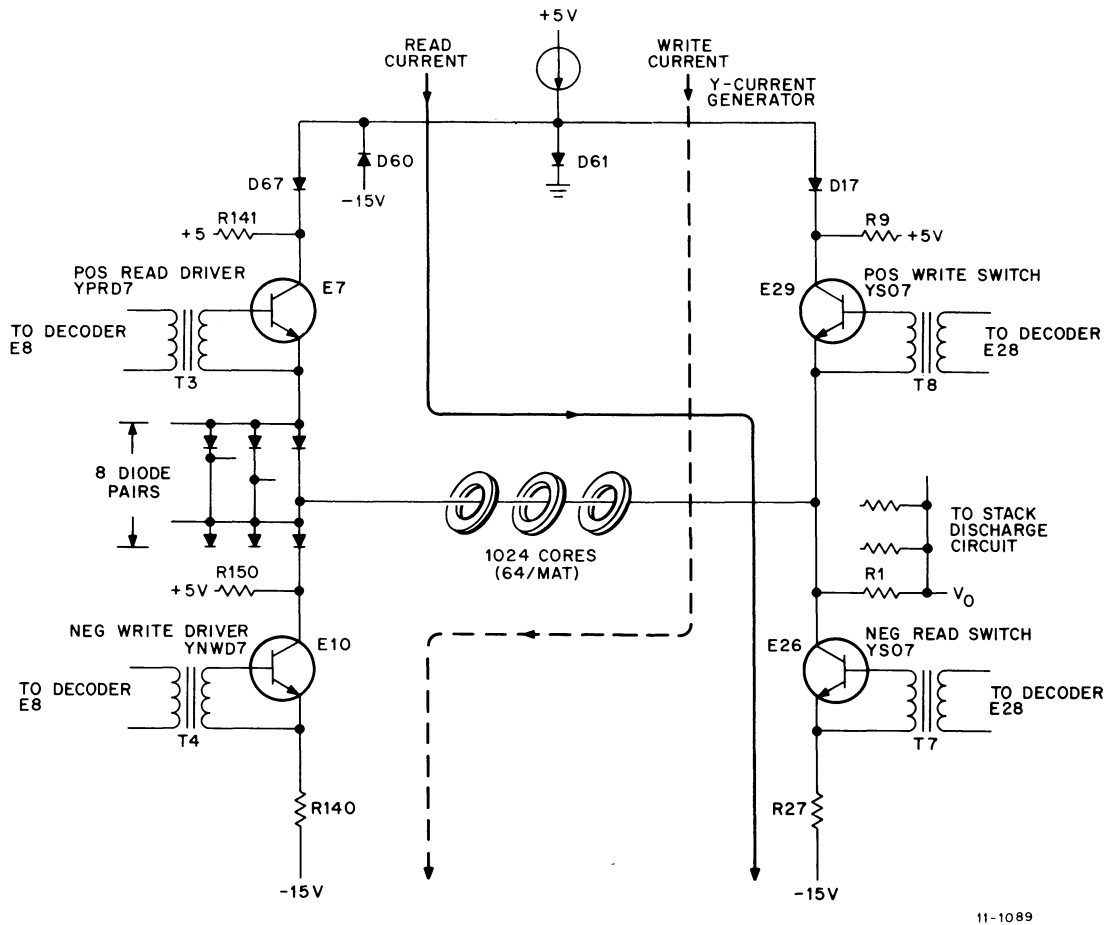
Figure 12-13 Typical Y-Line Read/Write Switches and Drivers
