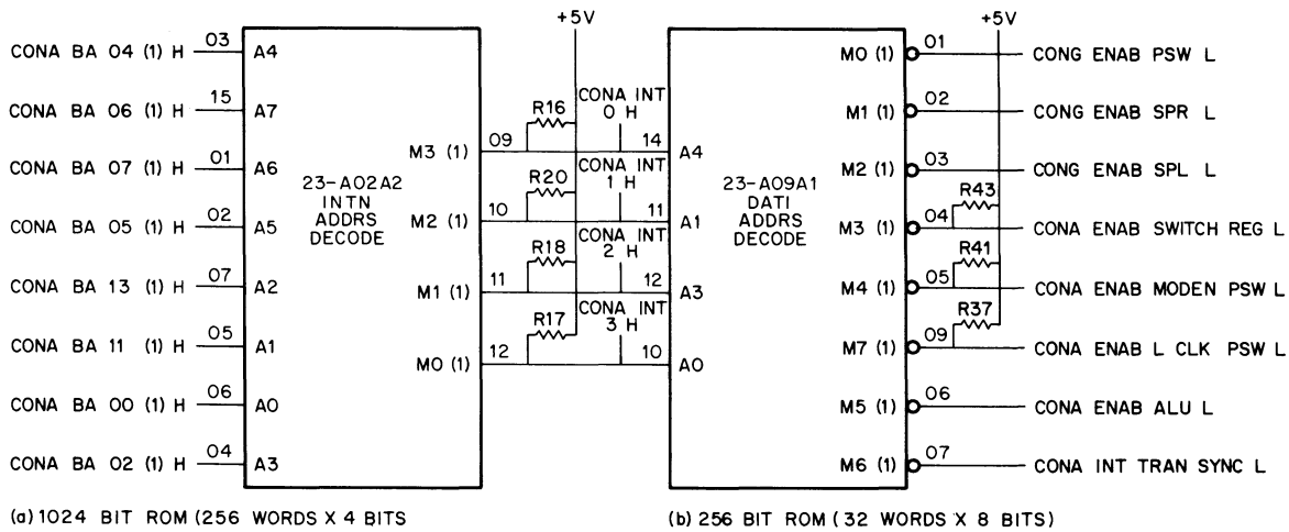
Figure 8-1 1024-Bit and 256-Bit ROMs
