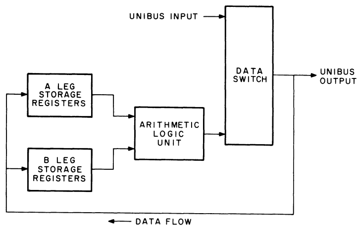
Figure 8-3 KD11-B Simplified Data Path Block Diagram
