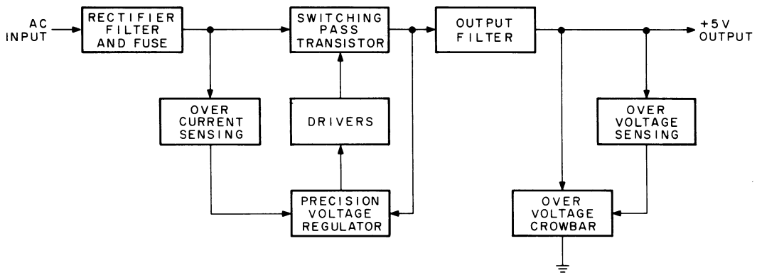
Figure 3-20 +5 V Regulator (PS2) Functional Block Diagram
