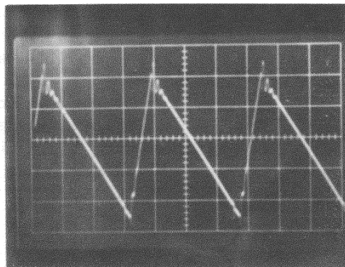
f) Point B, 20A load, \mu s/div, and 50 mV/div.
