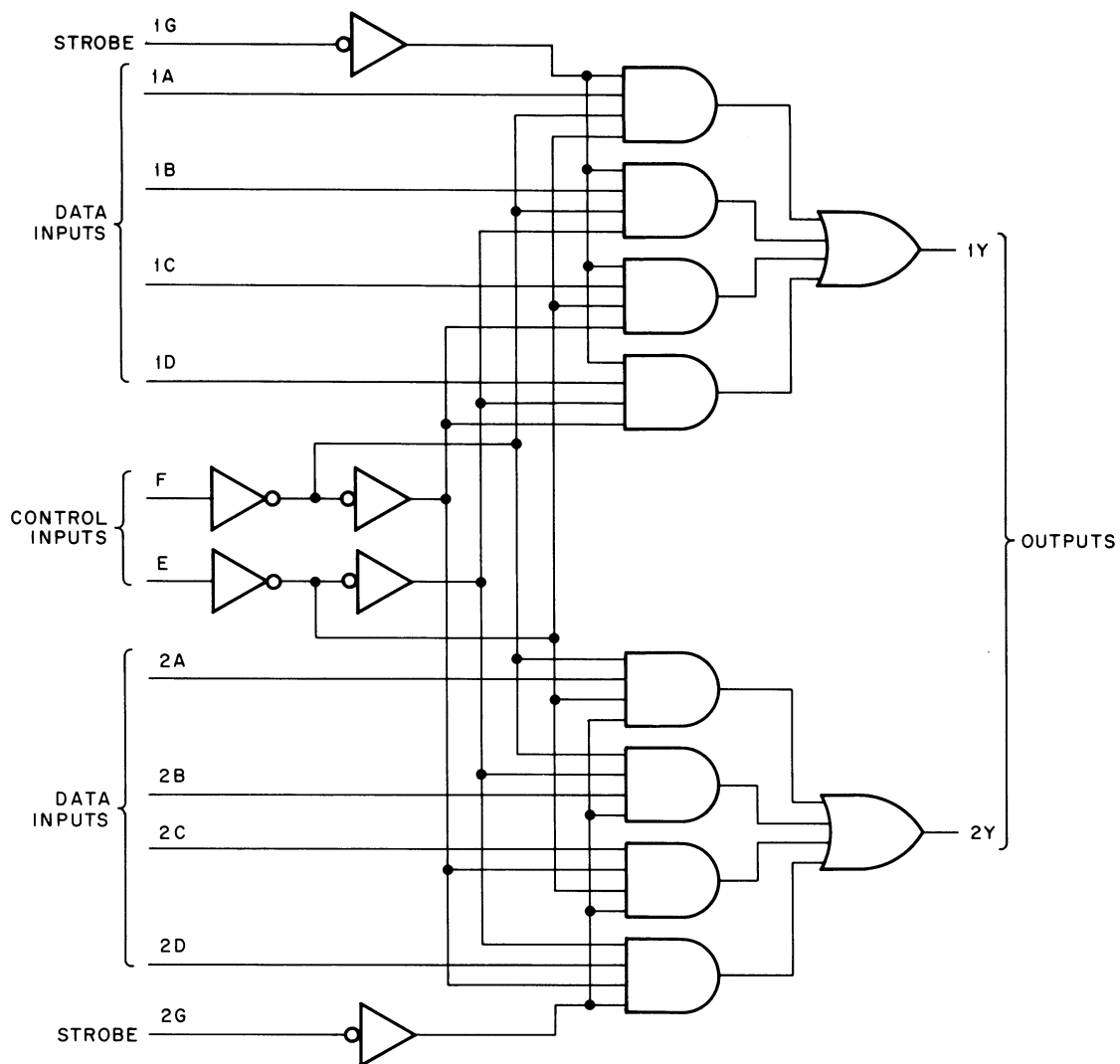
LOGIC DIAGRAM
