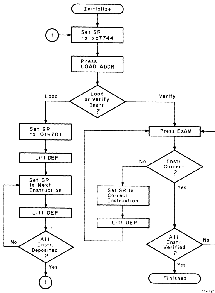
Figure 4-2 Loading and Verifying the Bootstrap Loader
