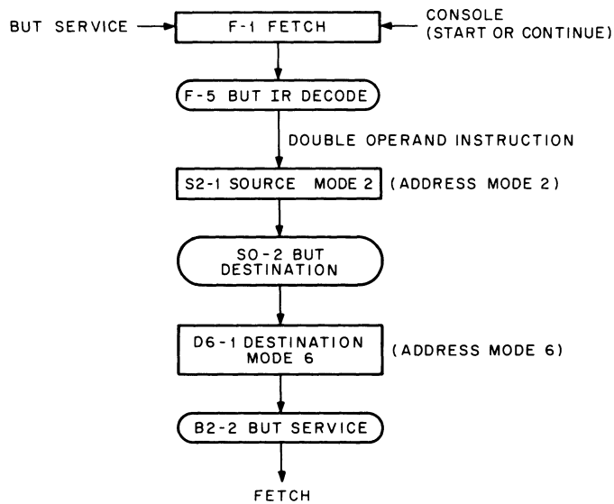
Figure 9-4 CMP # 15, CHAR (022767), Simplified Flow Diagram
