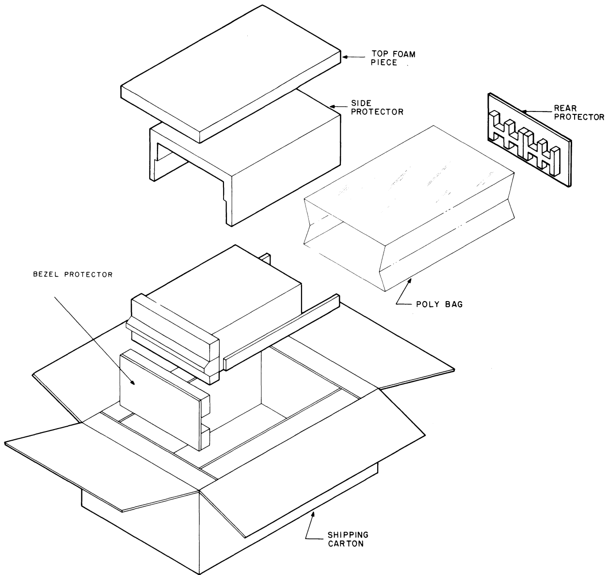
Figure 2-1 Computer Packaging
