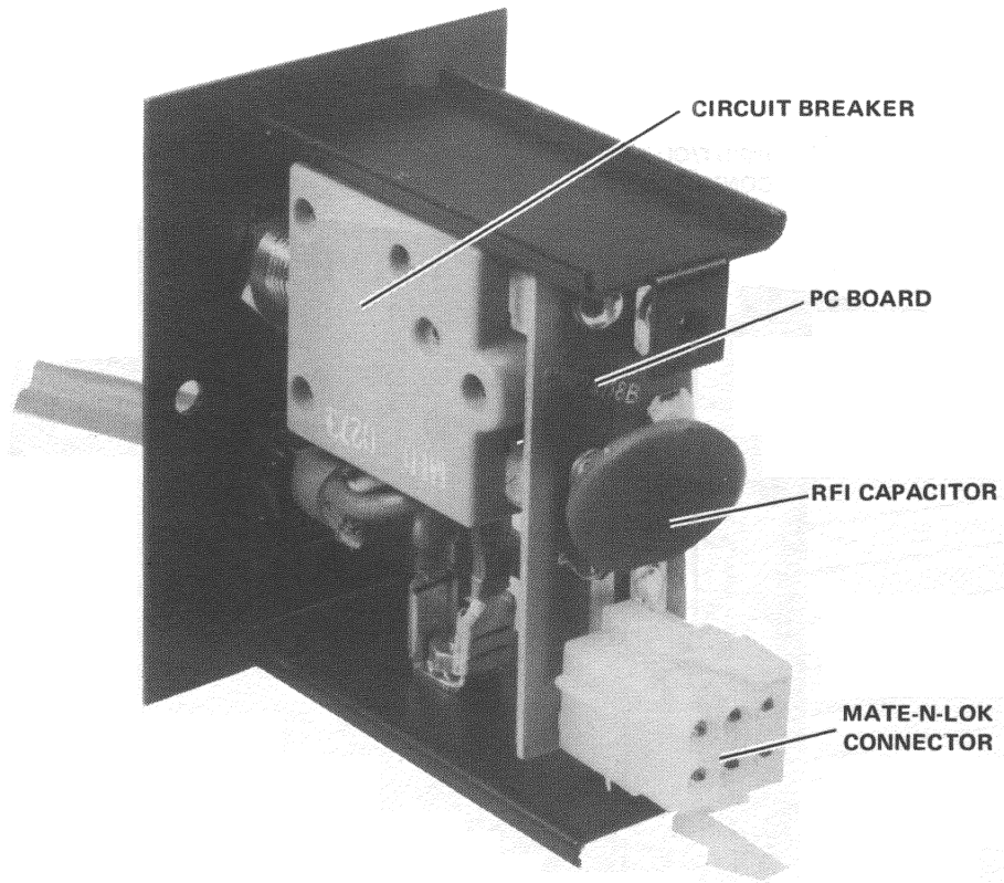
Figure 3-7 BC05T Line Set, Cover Removed
