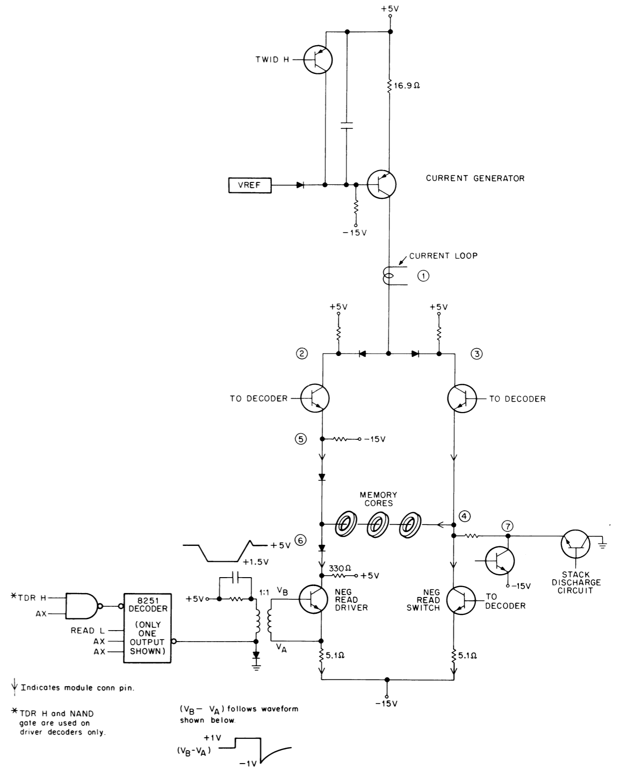
Figure 13-4 Drive Waveforms
