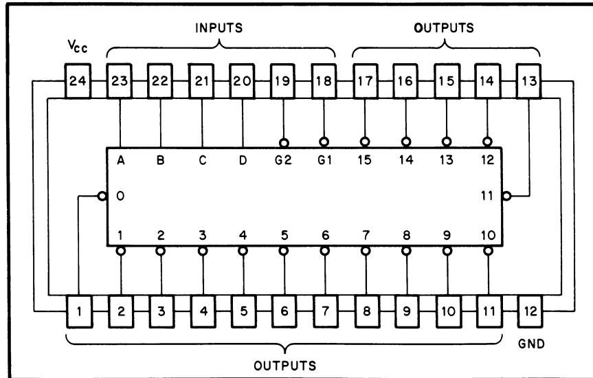
DUAL-IN-LINE PACKAGE (TOP VIEW)
