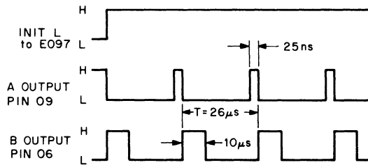
TIMING DIAGRAM
