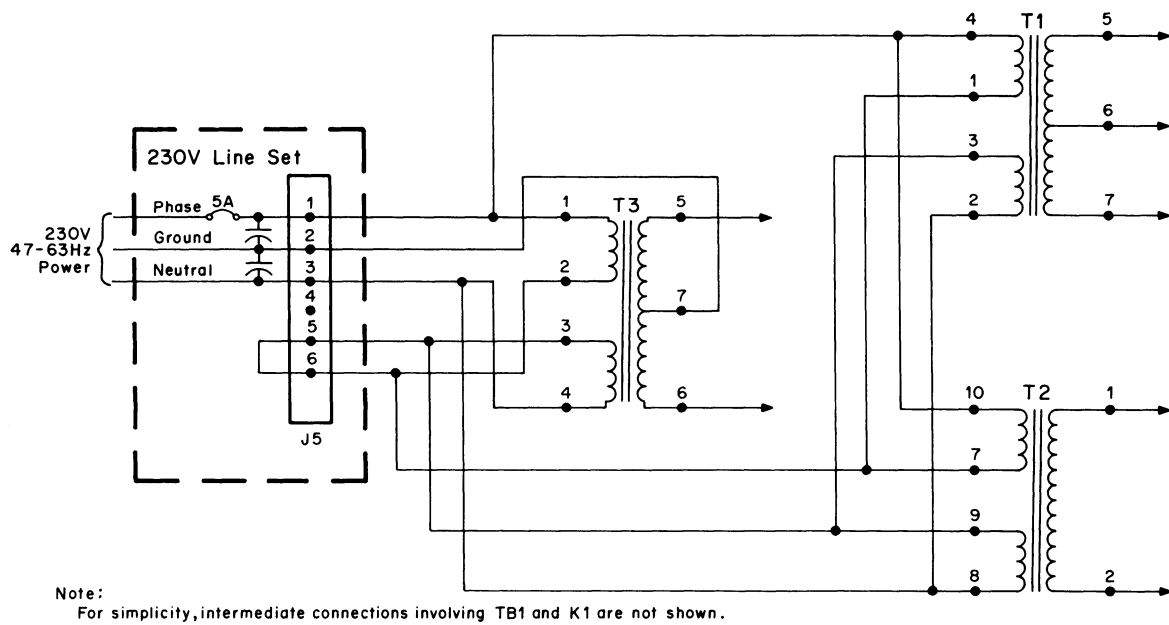
Figure 3-12 Power Application Using 230 V Line Set
