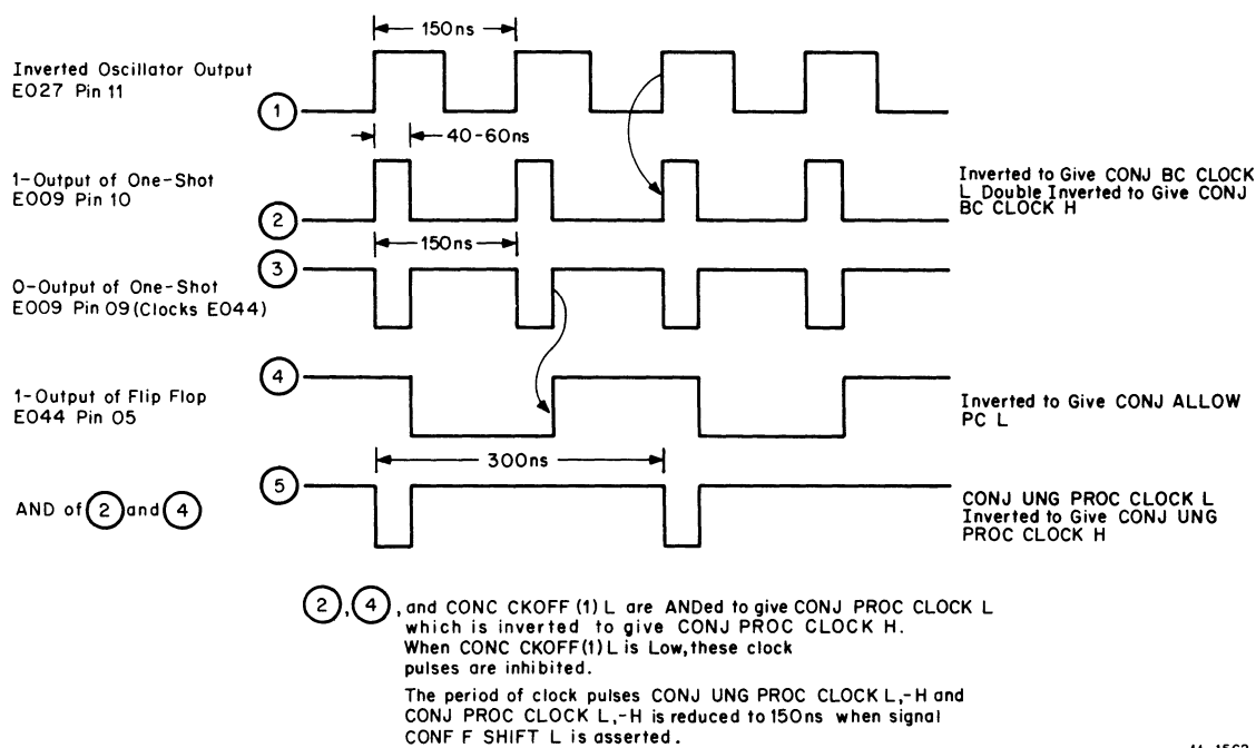
Figure 8-14 Processor Clock Timing Diagram
