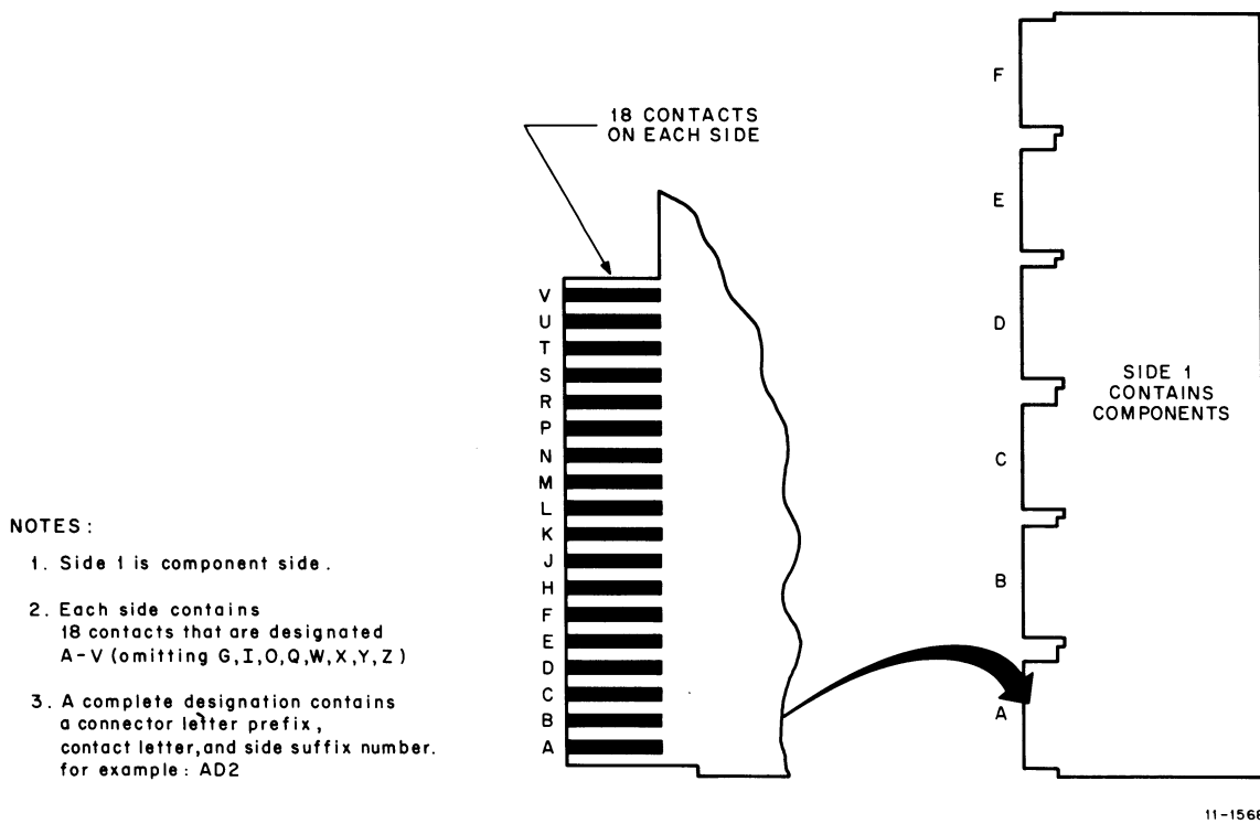
Figure 1-4 Module Contact Designations
