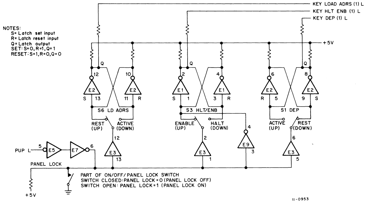
Figure 7-6 Control Switches and Bounce Buffers, Logic Diagram
