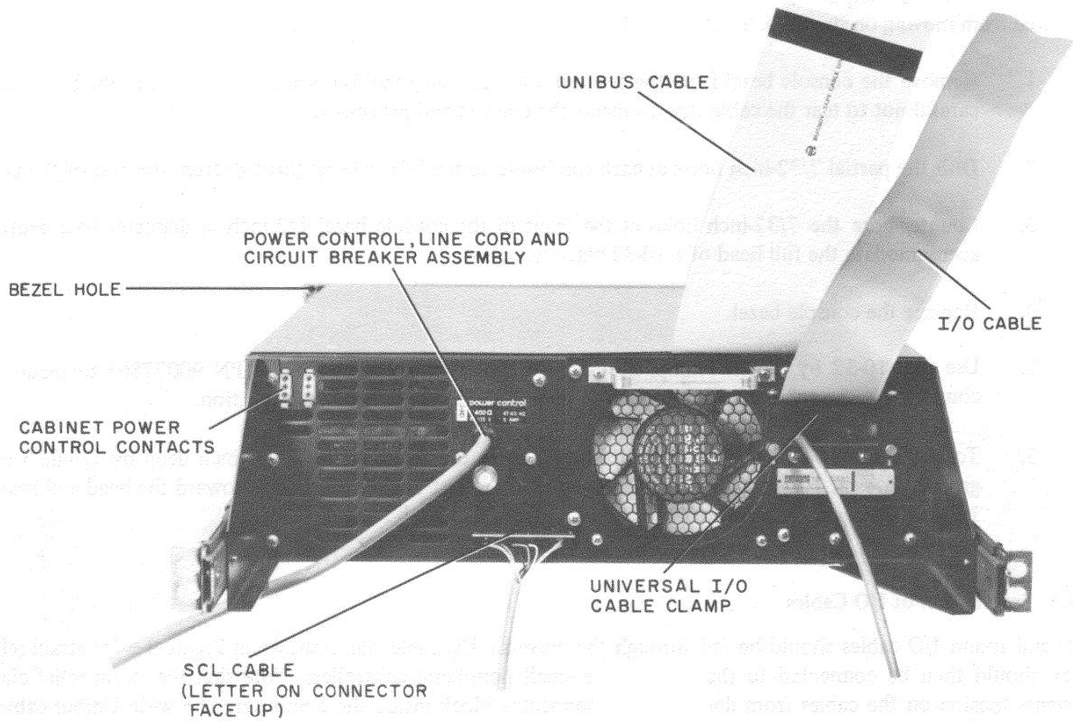
Figure 3-6 Mounting Box Without Modules
