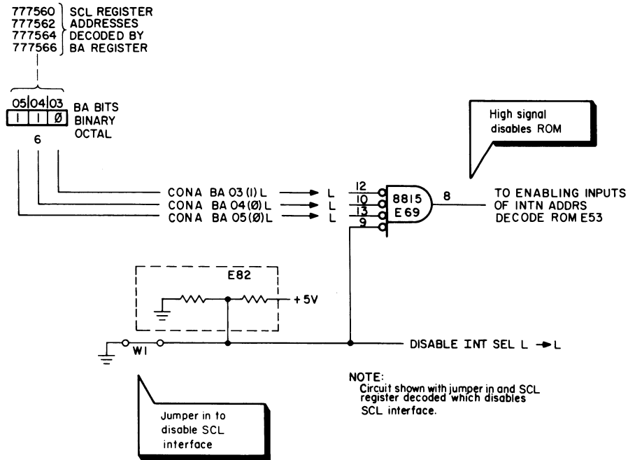
Figure 2 SCL Interface Disabling Circuit
