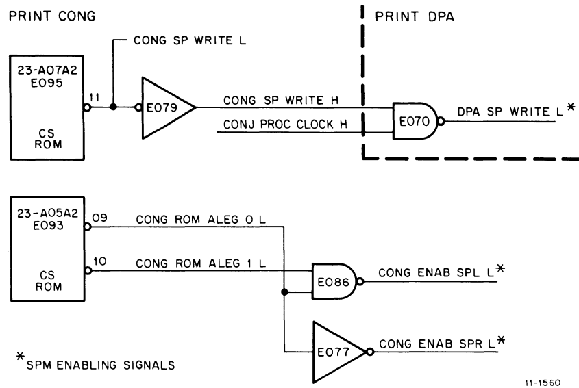
Figure 9-7 Generation of SPM Enabling Signals
