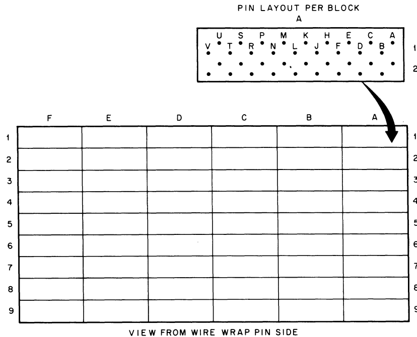
Figure 1-3 Computer Backplane Connector and Pin Designations
