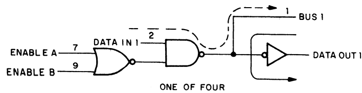
Figure 2 8838 Quad Bus Transceivers
