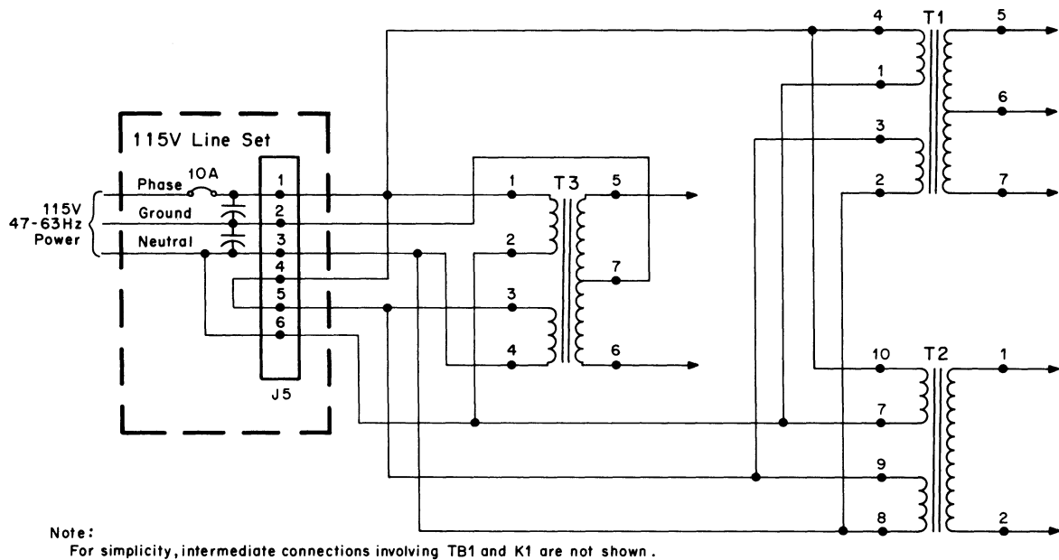
Figure 3-11 Power Application Using 115 V Line Set
