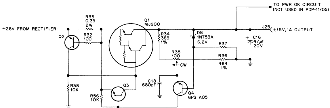
Figure 15-7 +15V Regulator Circuit
