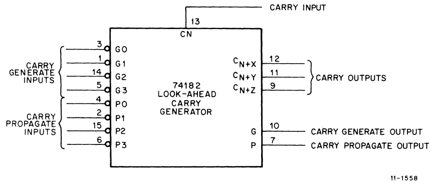
Figure 8-6 74182 Pin and Signal Designations
