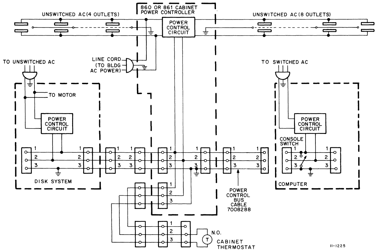
Figure 2-3 Typical Cabinet Power Control System Wiring Diagram
