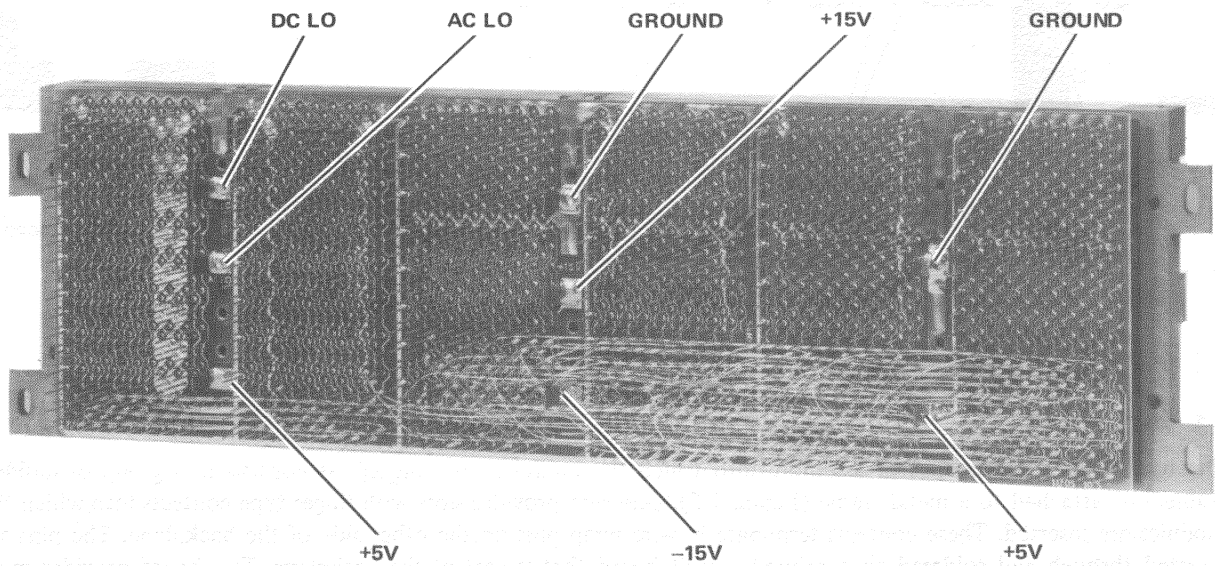
Figure 1-6 Pin Side of Backplane
