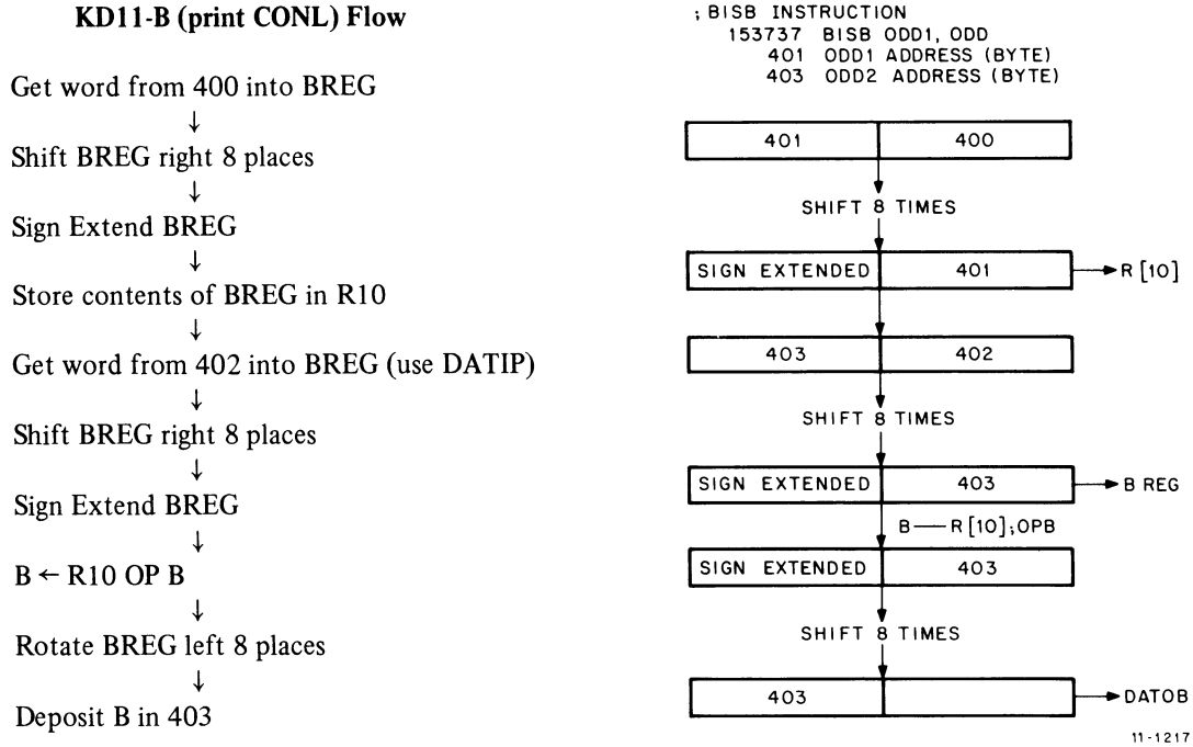
Figure 8-10 Byte Format for Shifting Instructions
