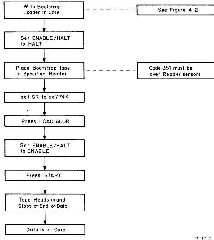
Figure 4-3 Loading Bootstrap Tapes Into Memory
