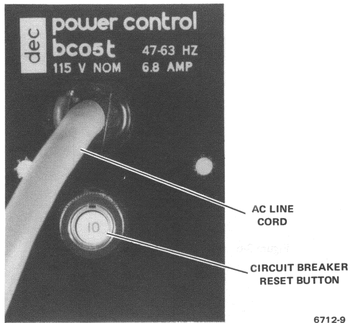
Figure 3-8 BC05T Line Set, Rear View
