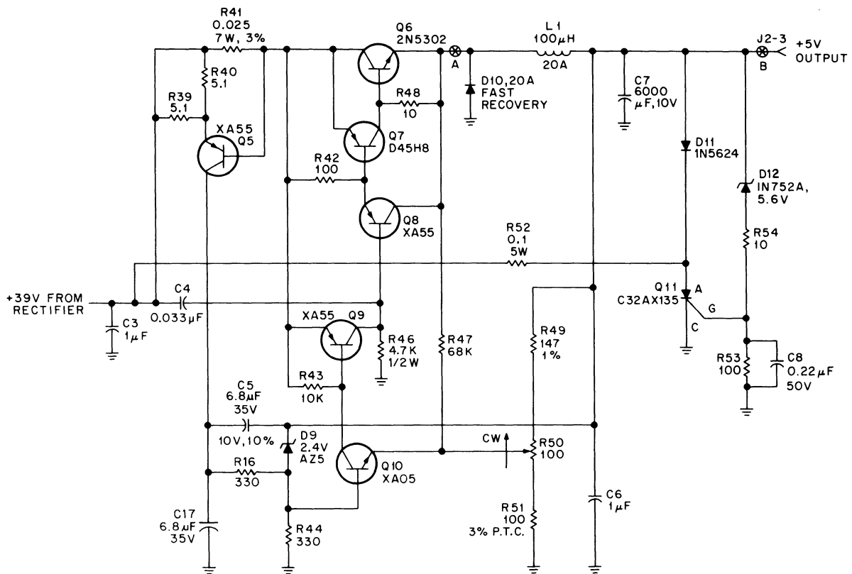
Figure 3-18 +5 V Regulator Circuit
