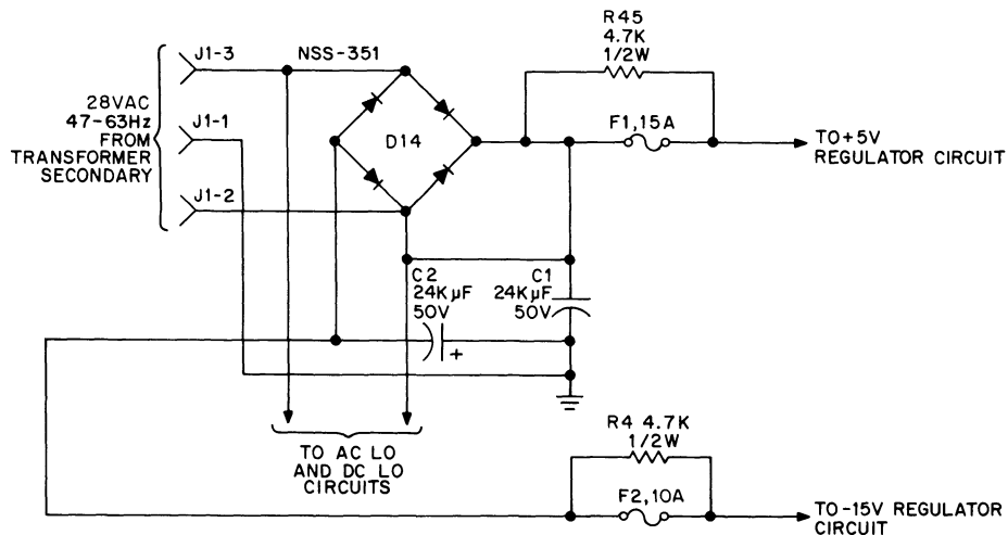
Figure 3-15 Rectifier and LTC Circuits
