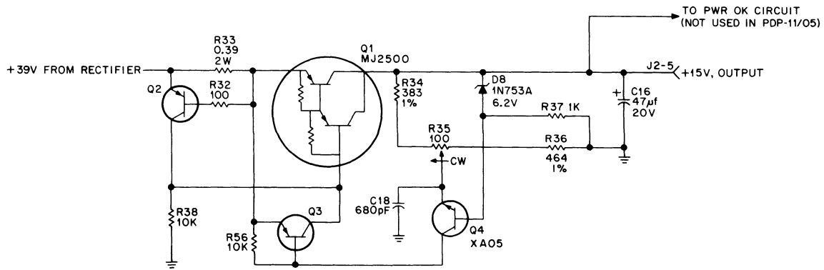
Figure 3-17 +15 V Regulator Circuit
