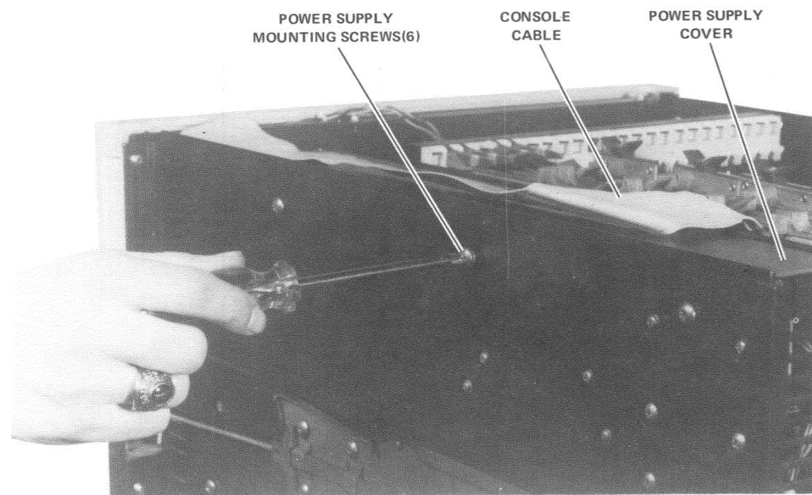
Figure 3-26 Removing Power Supply Mounting Screws
