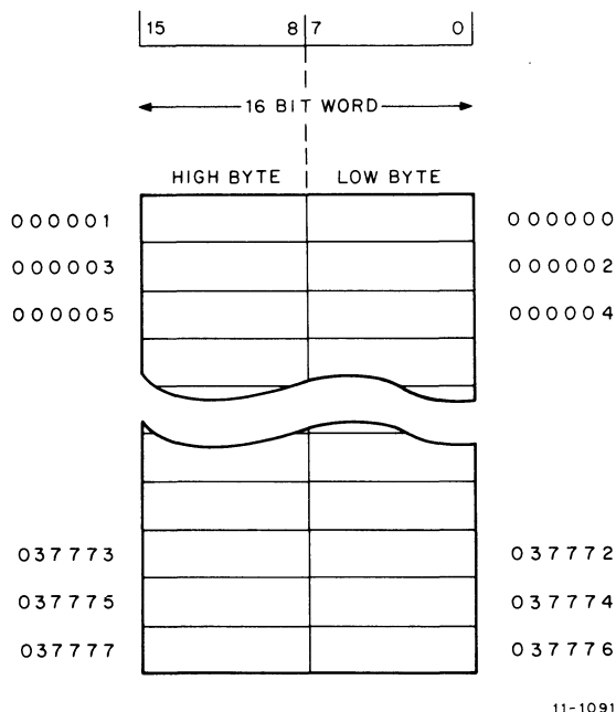
Figure 12-5 Memory Organization for 8K Words
