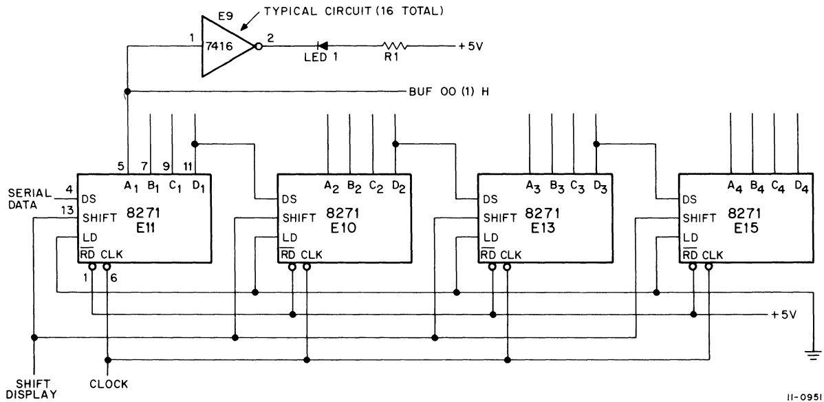
Figure 7-4 Display Buffer and Driver, Simplified Logic Diagram
