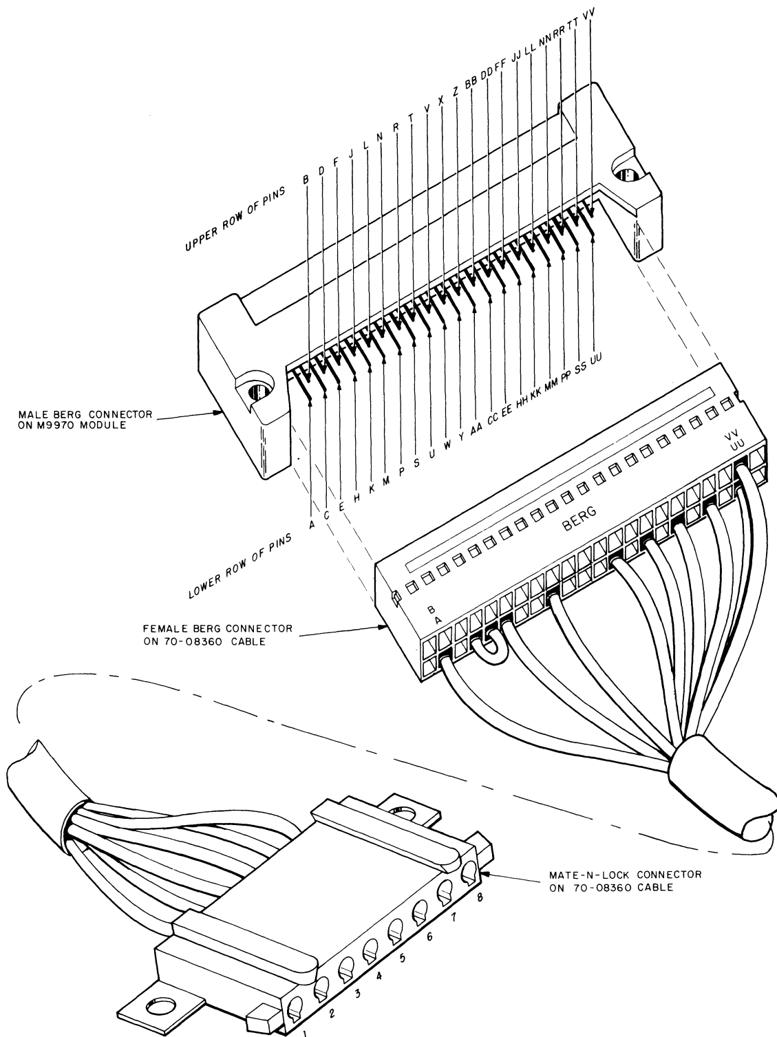
Figure B-1 SCL Cable 70-08360
