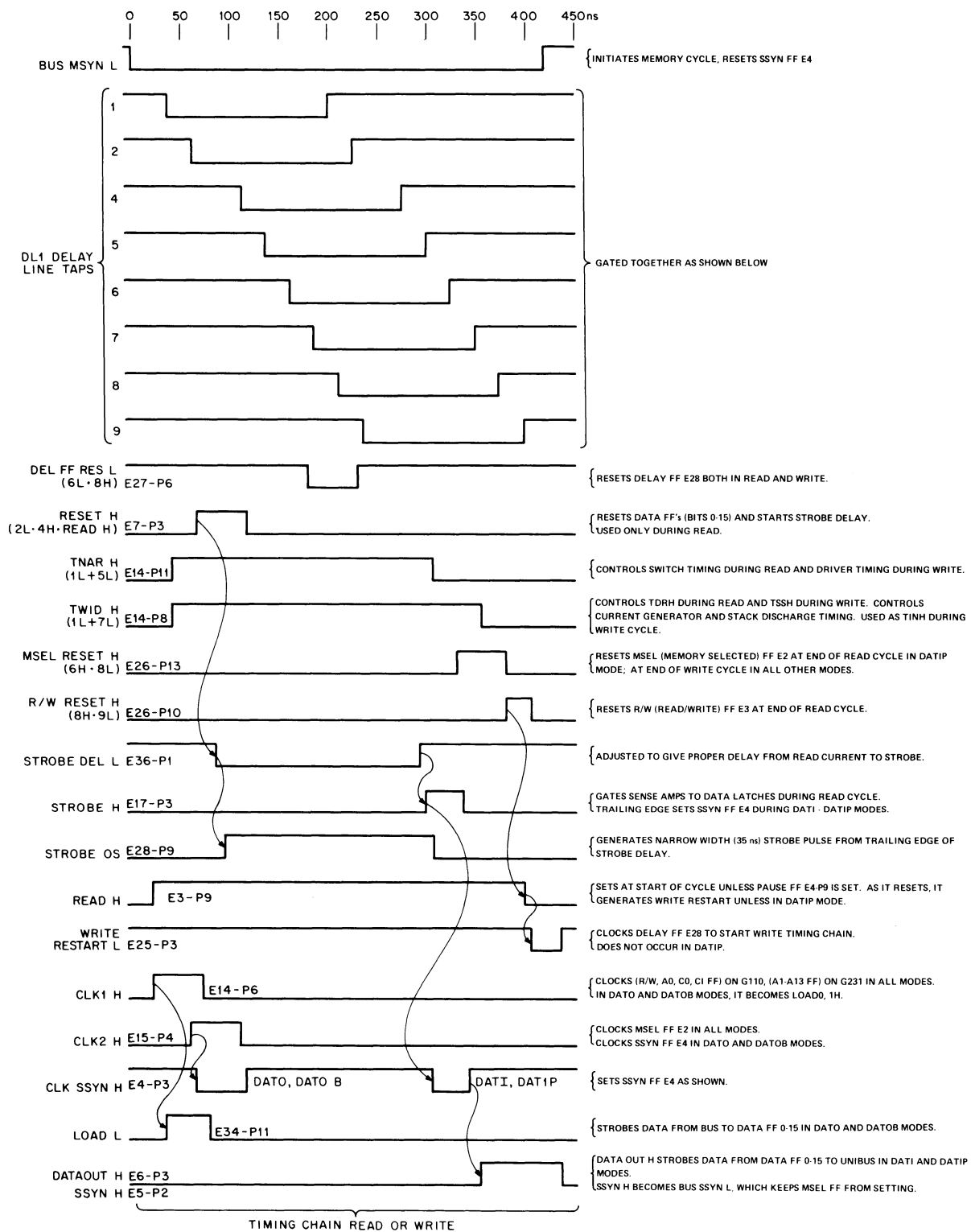
Figure 12-20 Basic Timing and Control Signal Functions
