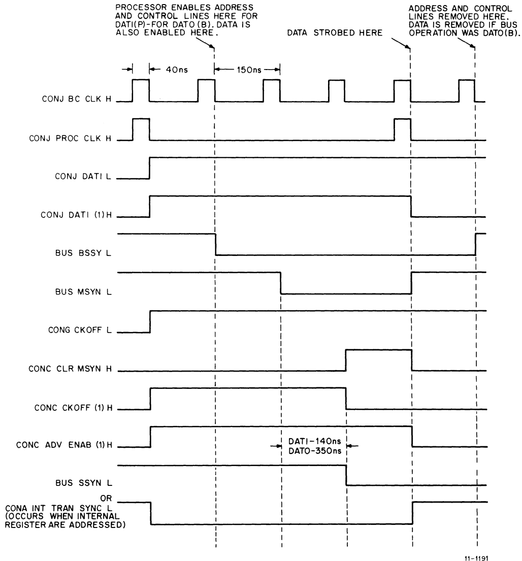
Figure 8-15 DATI and DATO Timing
