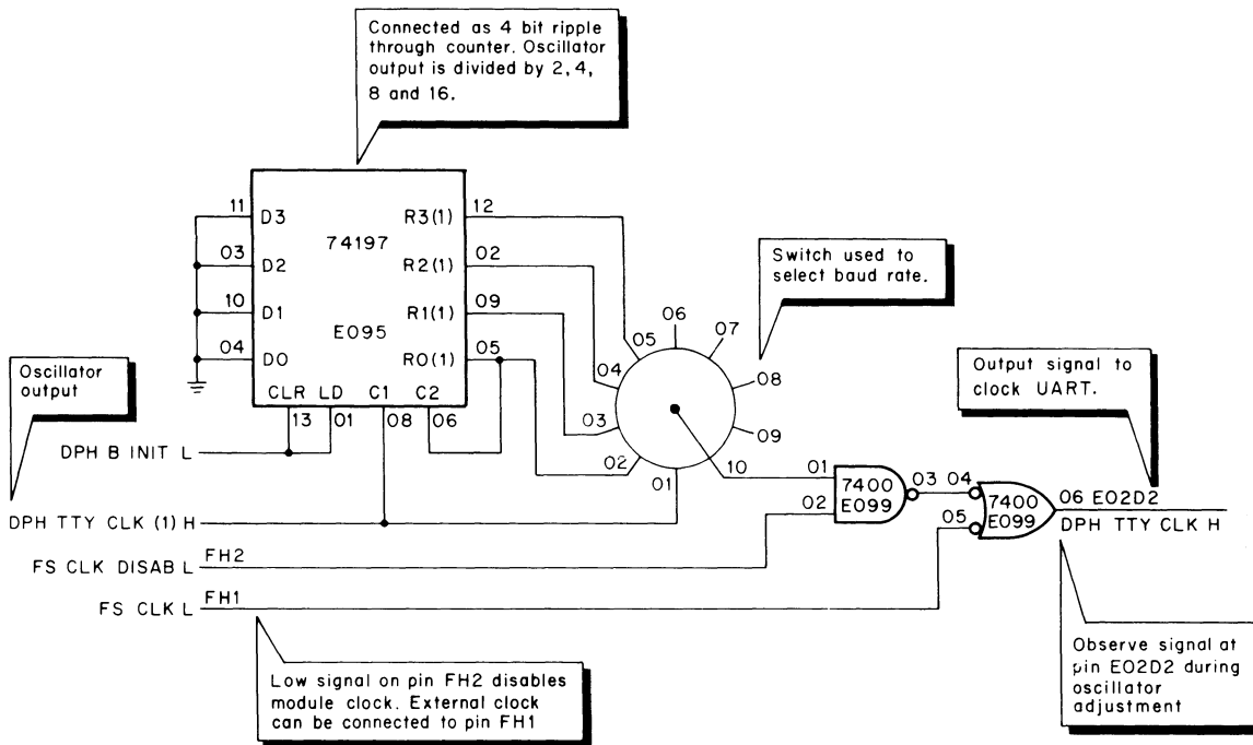
Figure 6 Baud Selection Logic
