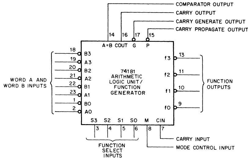
Figure 8-5 74181 Pin and Signal Designations
