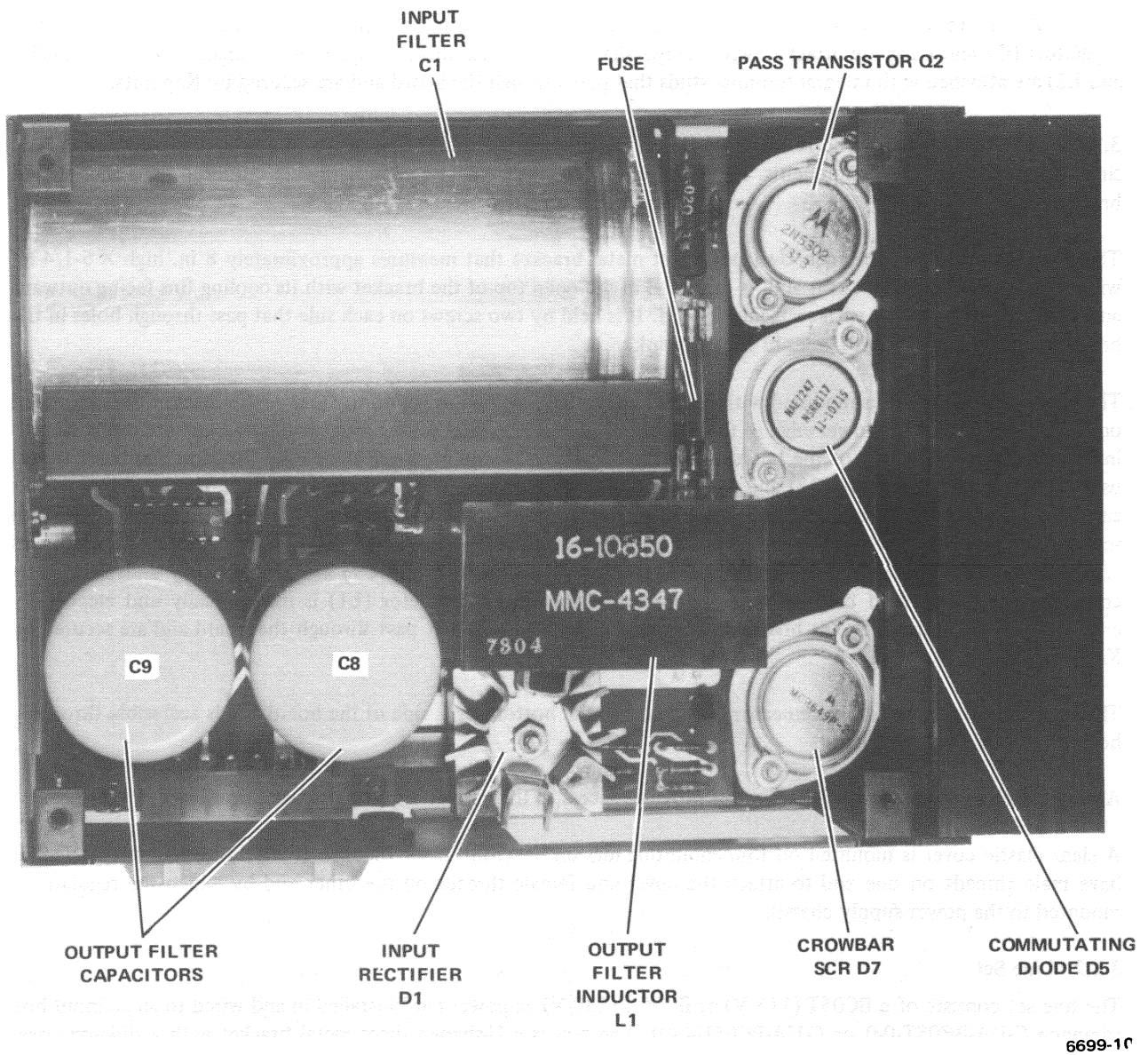
Figure 3-5 +5 V Regulator, Side View
