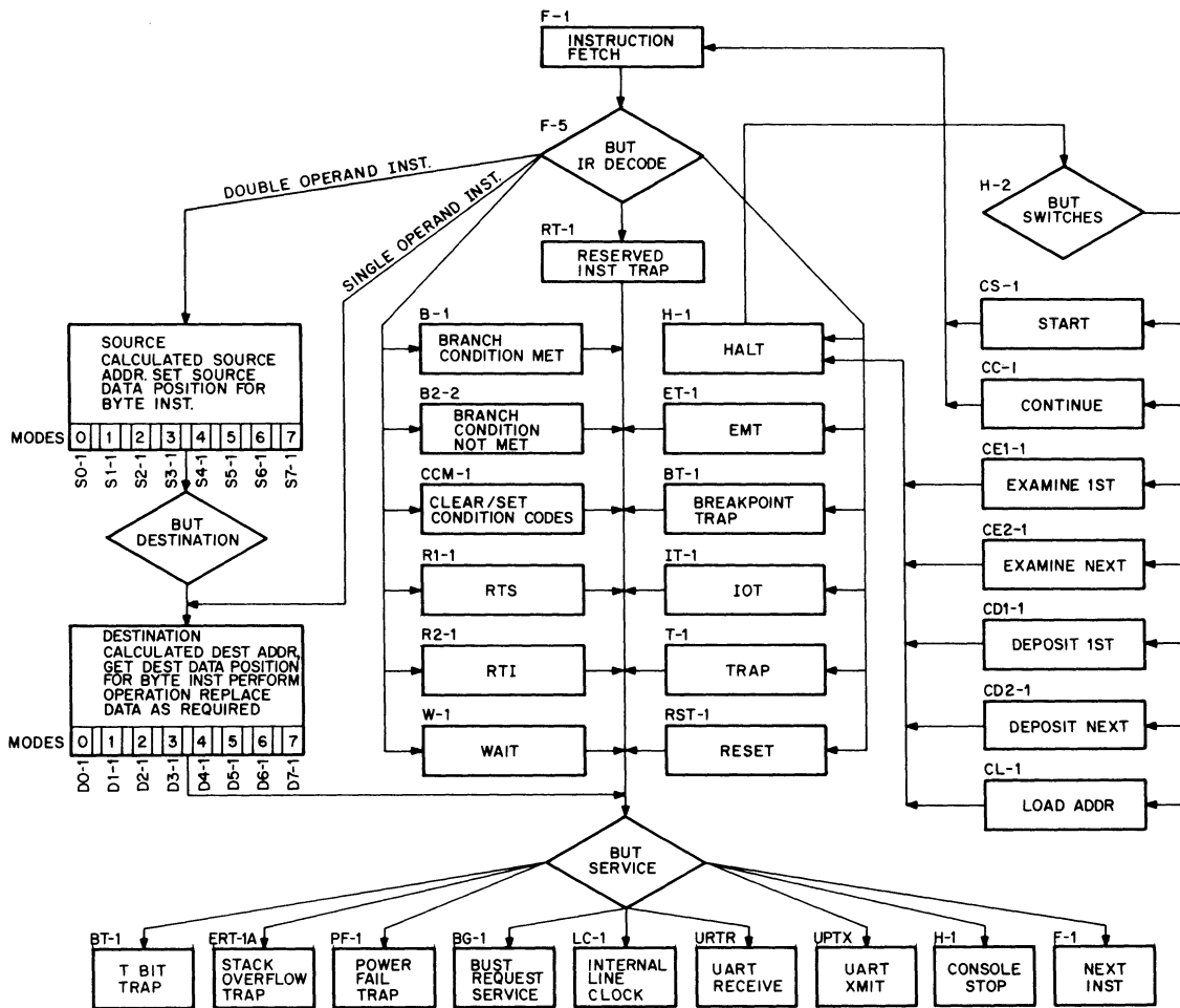
Figure 9-2 KD11-B Simplified Flow Diagram
