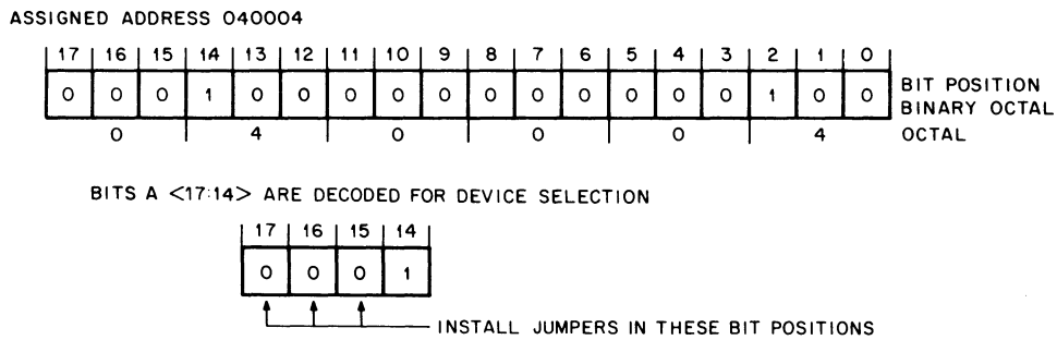
Figure 12-7 Jumper Configuration For A Specific Memory Address
