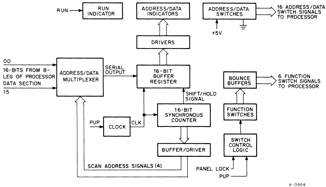
Figure 7-1 Console Functional Block Diagram
