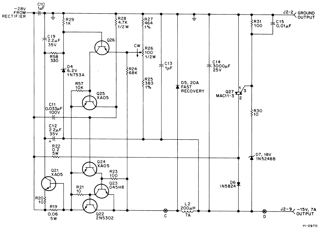
Figure 15-9 -15V Regulator Circuit
