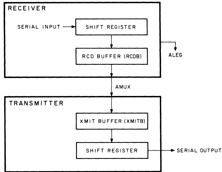
Figure 8-18 Double-Buffering Data Flow
