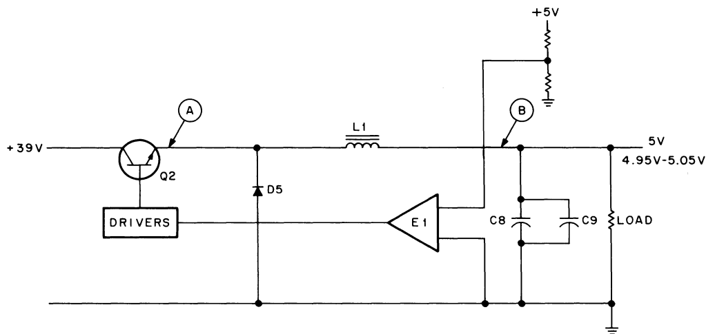
Figure 3-23 Simplified 5 V Switching Regulator Schematic and Waveforms
