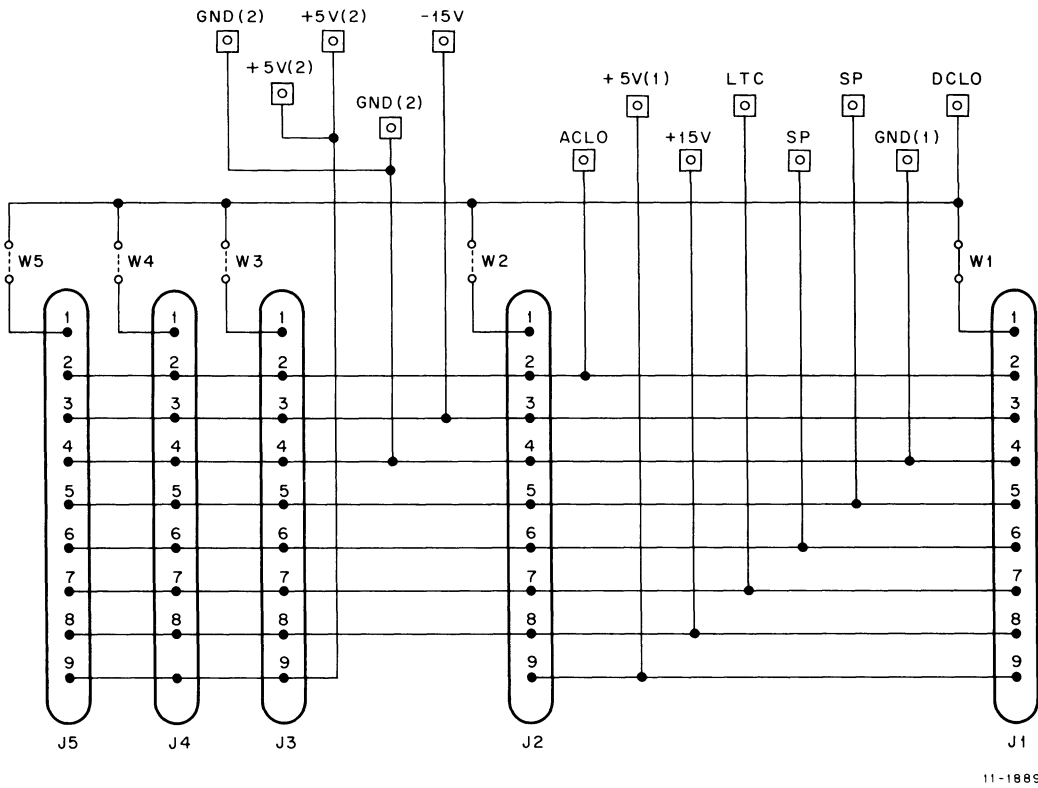
Figure 3-13 Power Distribution Board Circuit Schematic
