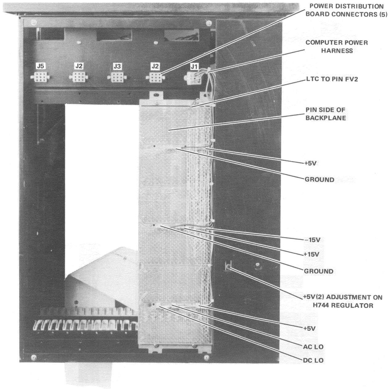
Figure 1-3 PDP-11/05 NC Computer Extended and Locked In Front Up 90° Position
