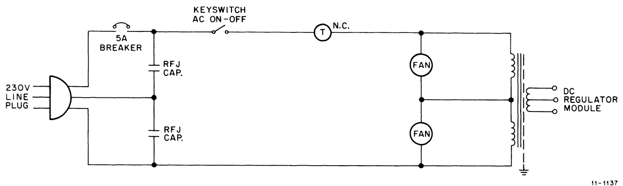
Figure 15-3 230V Connection Diagram
