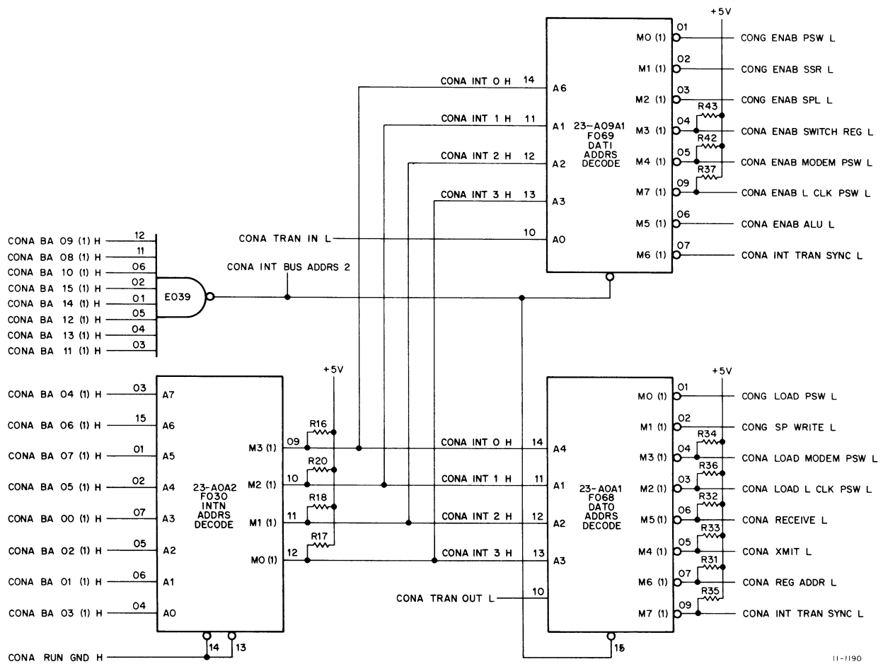
Figure 8-16 Unibus Address Decoding
