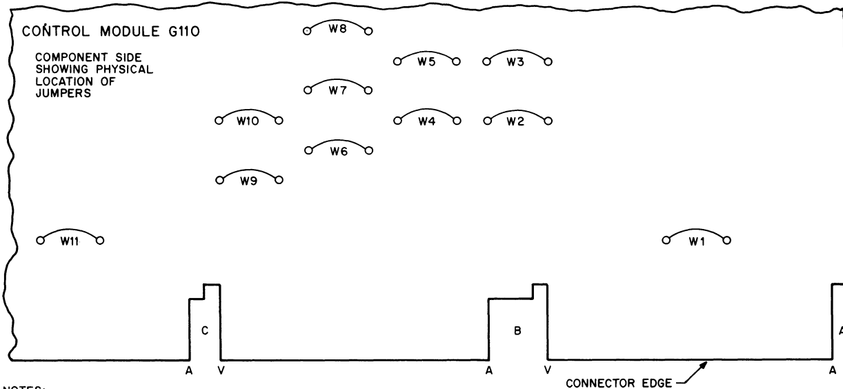
Figure 12-7 Jumper Configuration For A Specific Memory Address
