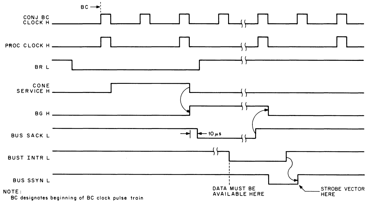
Figure 8-17 Bus Request (BR) Timing
