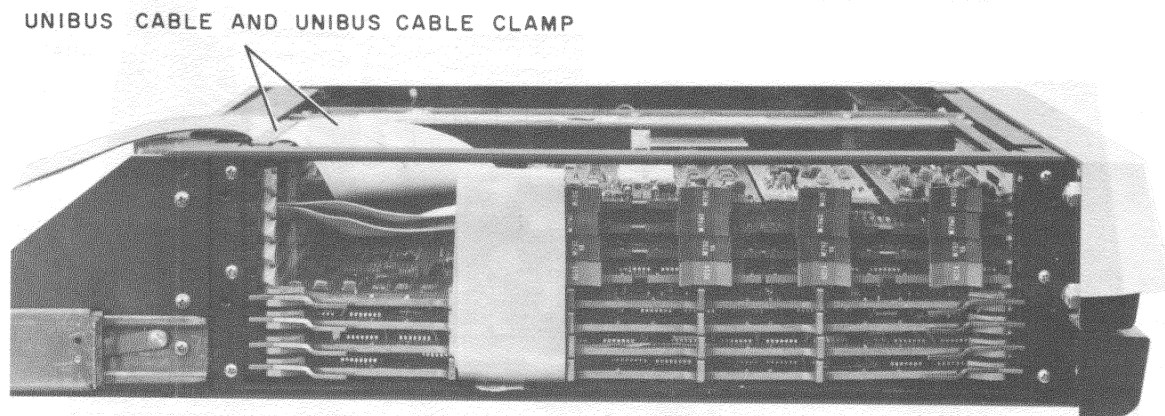
Figure 3-5 Computer Chassis (showing peripheral cables and the Unibus)
