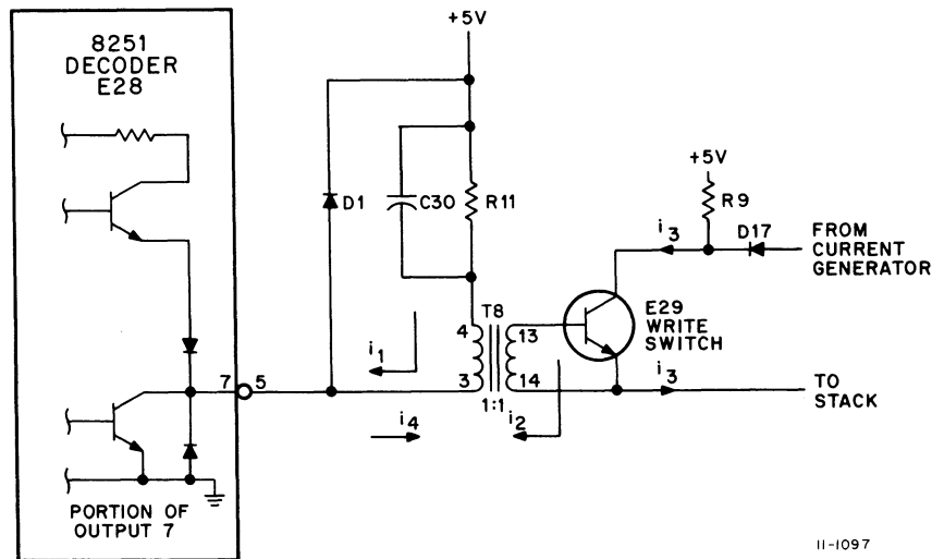
Figure 12-11 Switch or Driver Base Drive Circuit
