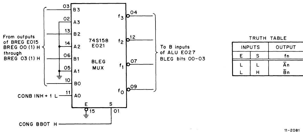
Figure 4 Multiplexer for BLEG Bits 00-03
