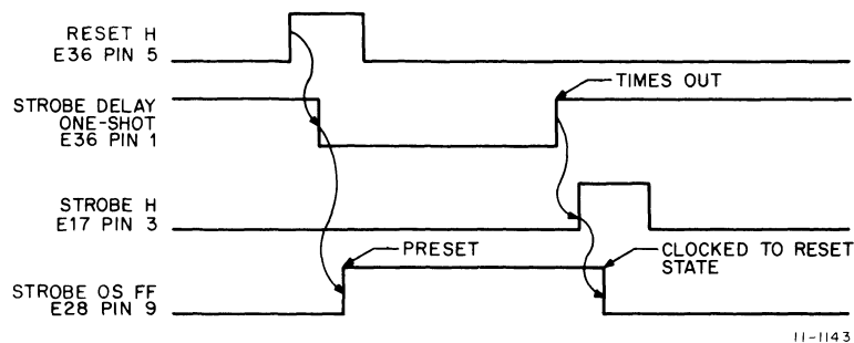
Figure 12-25 Strobe Generating Circuit and Timing Diagram for STROBE H
