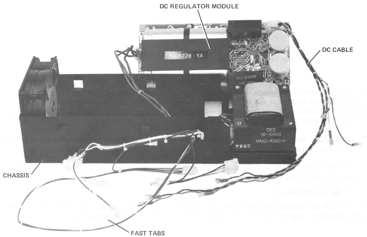
Figure 14-4 DC Regulator Module (Bottom View In Mounting Box)
