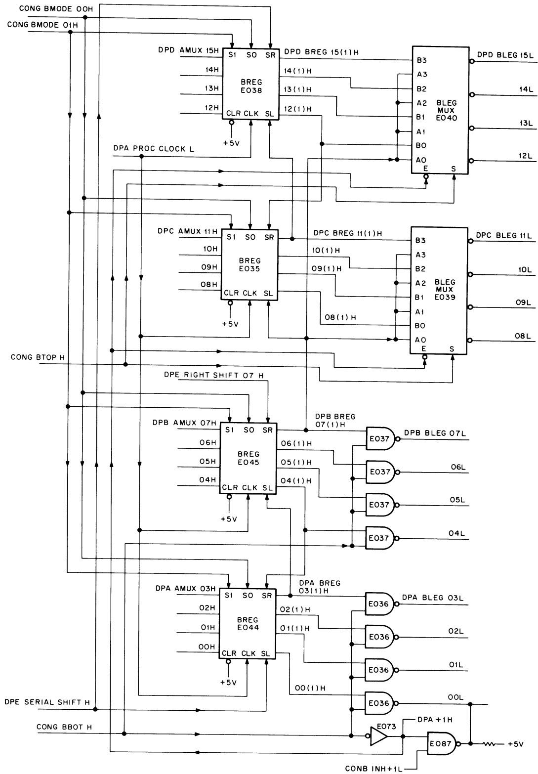
Figure 8-8 B Register and Output Logic
