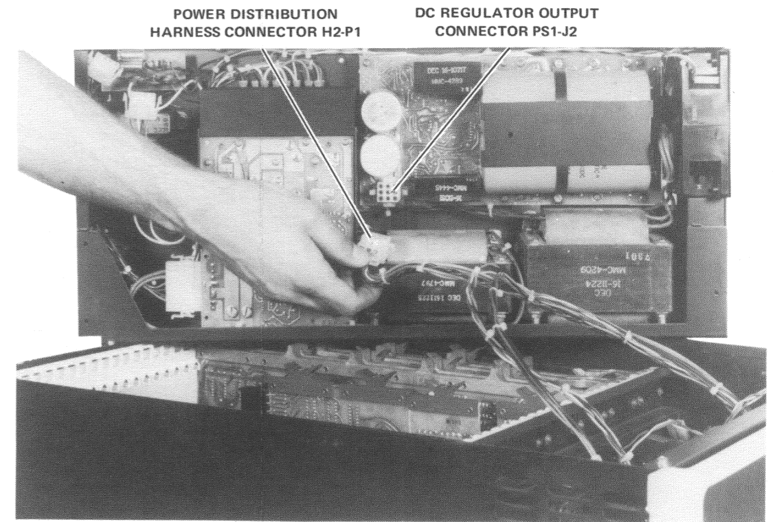
Figure 3-29 Disconnecting DC Regulator Output Connector
