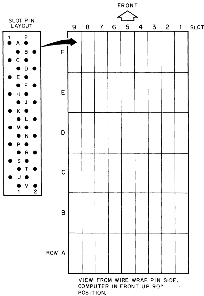
Figure 1-7 Computer Backplane Connector and Pin Designations
