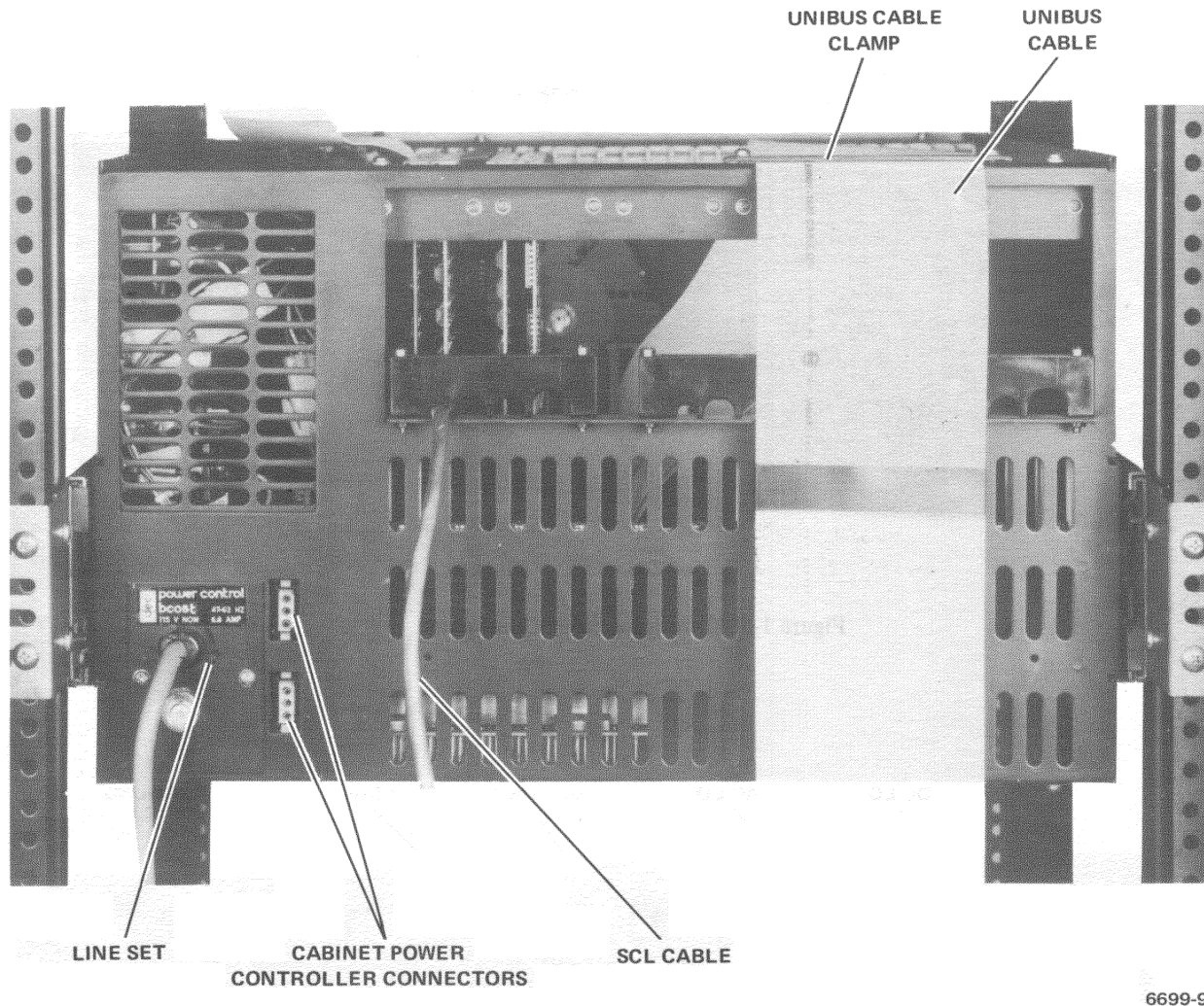
Figure 1-4 PDP-11/05 NC Computer, Rear View
