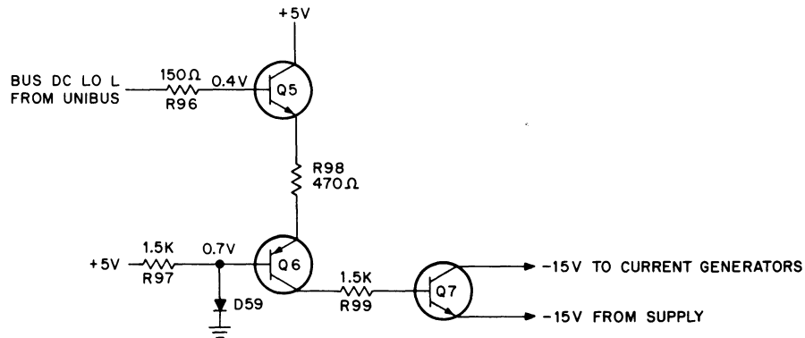
Figure 12-19 DC LO Circuit, Schematic Diagram
