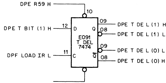
b) Typical 7474 Flip-Flop
