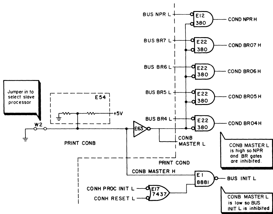
Figure 3 Slave Processor Selection Circuit
