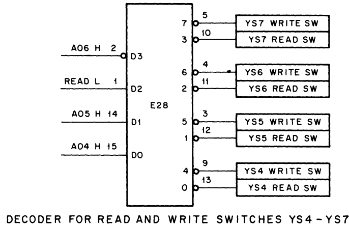
DECODER FOR READ AND WRITE SWITCHES YS4 - YS7
