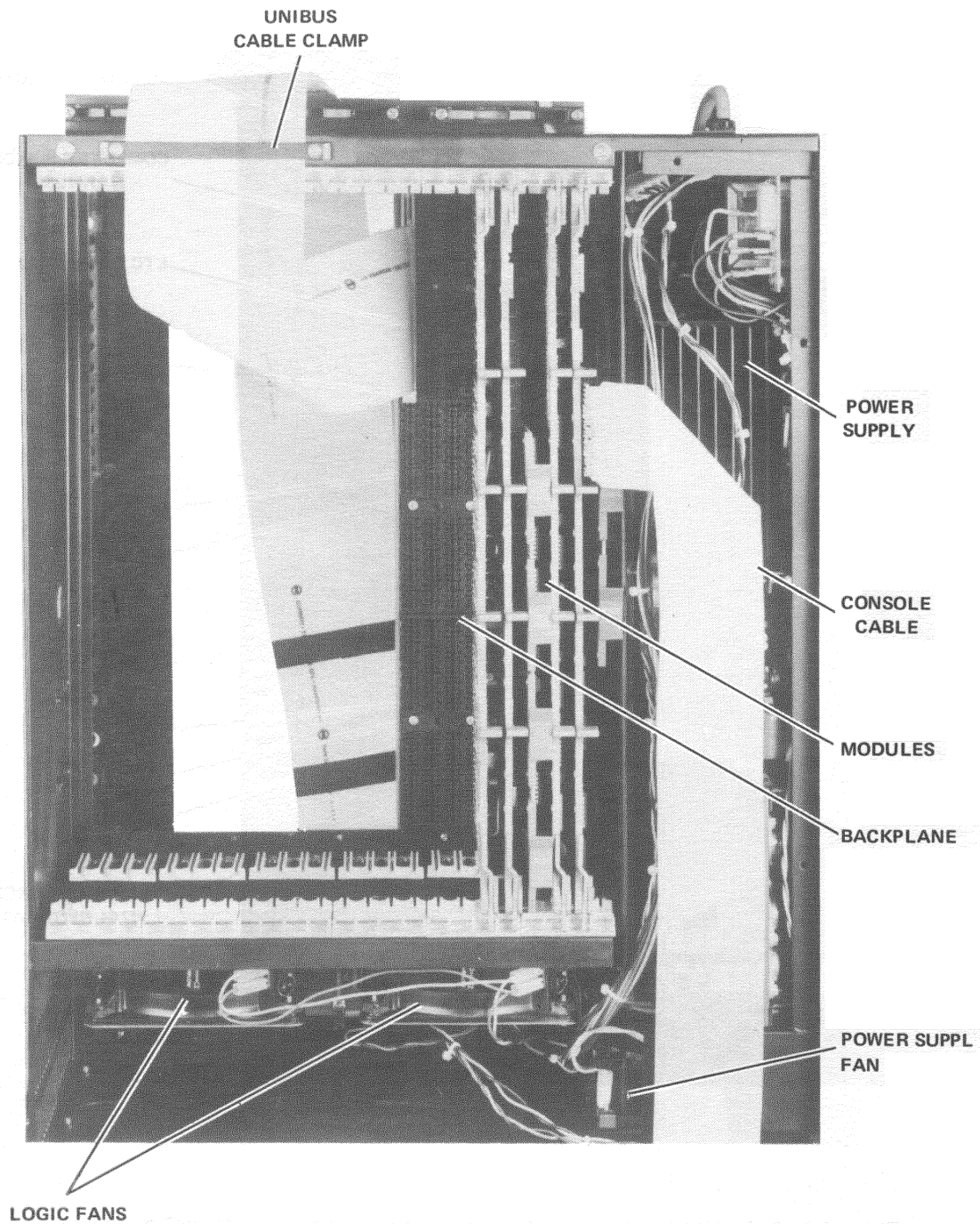
Figure 1-2 PDP-11/05 NC Computer Extended and Locked In Front Down 90° Position
