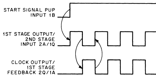
Figure 7-2 Console Clock, Schematic and Timing Diagram
