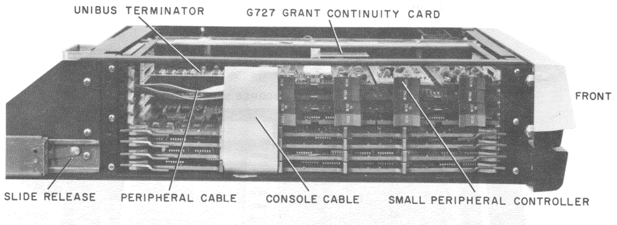
Figure 3-4 Computer Box with Top and Side Covers Removed
