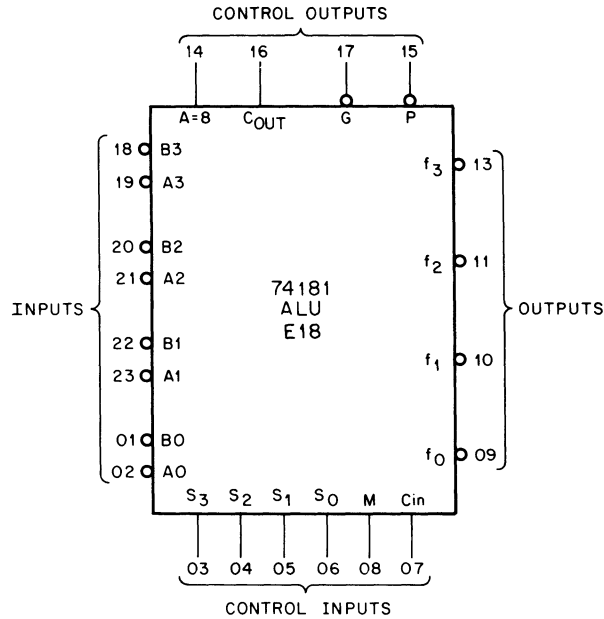
Figure 5-6 ALU, MSI Circuit Type 74181 Representation
