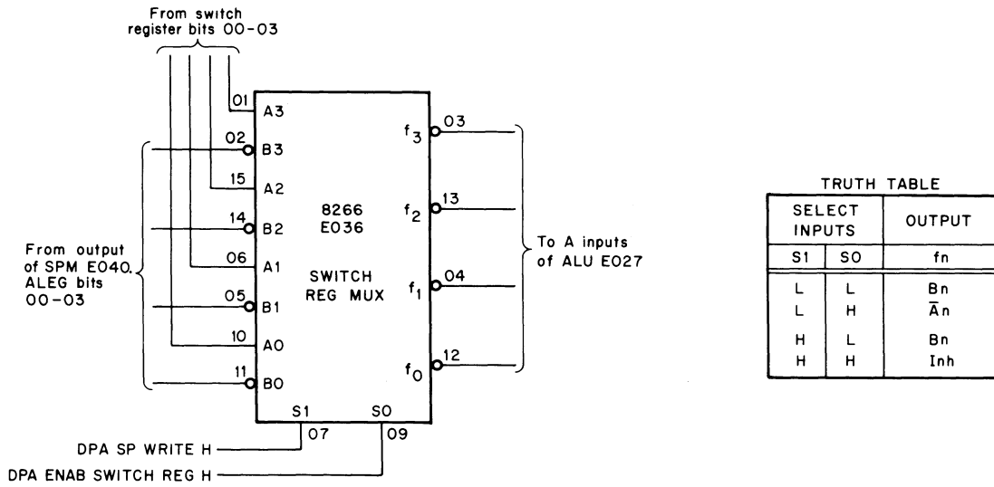
Figure 3 Typical Switch Register Multiplexer
