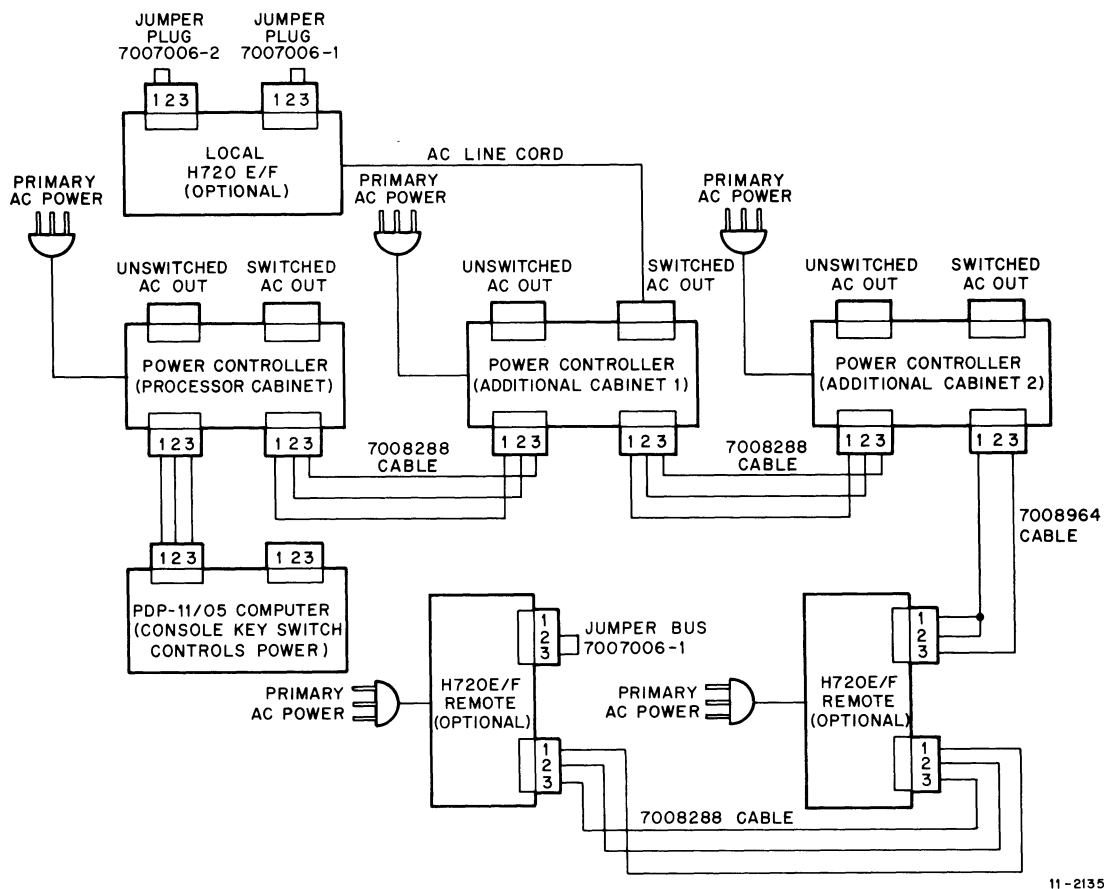
Figure 2-4 Interconnection of Power Controllers in Multi Cabinet Installation
