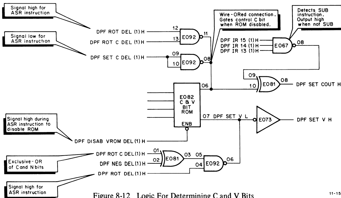
Figure 8-12 Logic For Determining C and V Bits (Example Shown for ASR Instruction)
