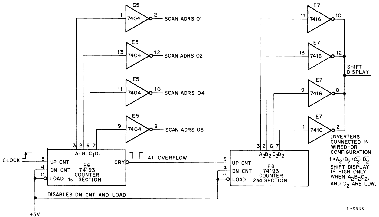
Figure 7-3 Counter, Simplified Logic Diagram
