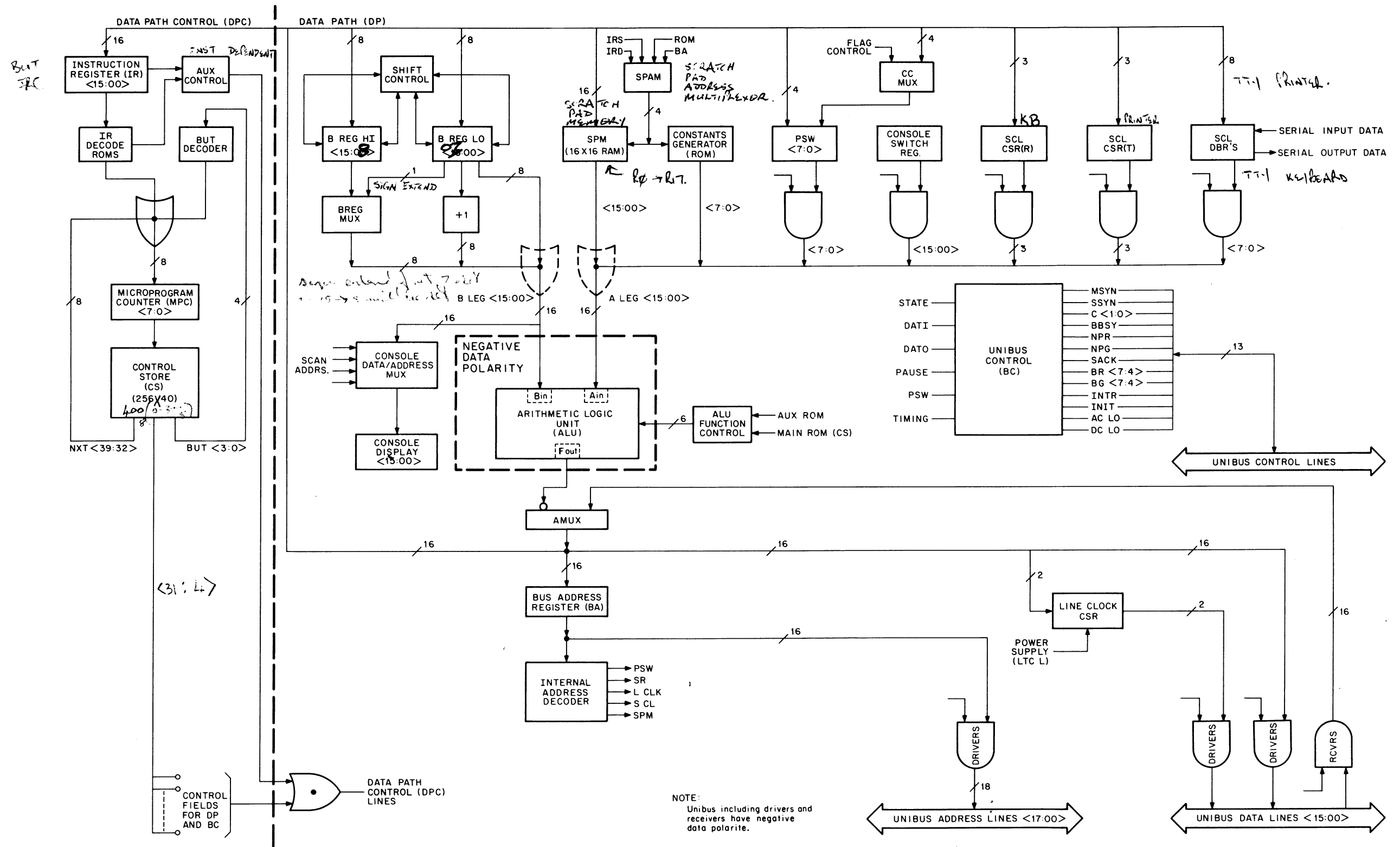
Figure 8-4 KD11-B Detailed Block Diagram
