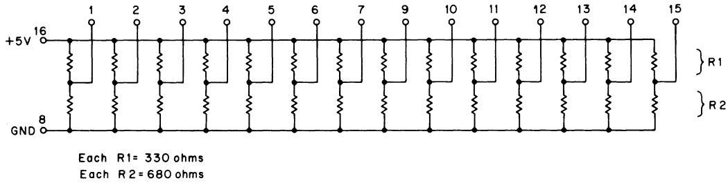
Circuit Schematic
