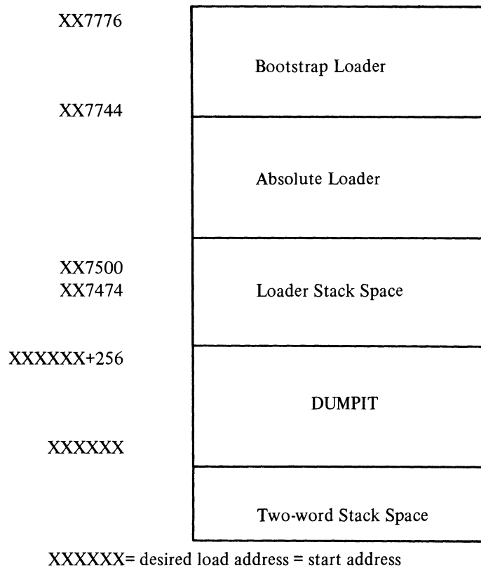
Figure 4-4 Absolute Format
