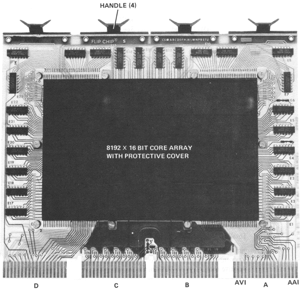
Figure 11-3 Component Side of 8K H214 Stack Module
