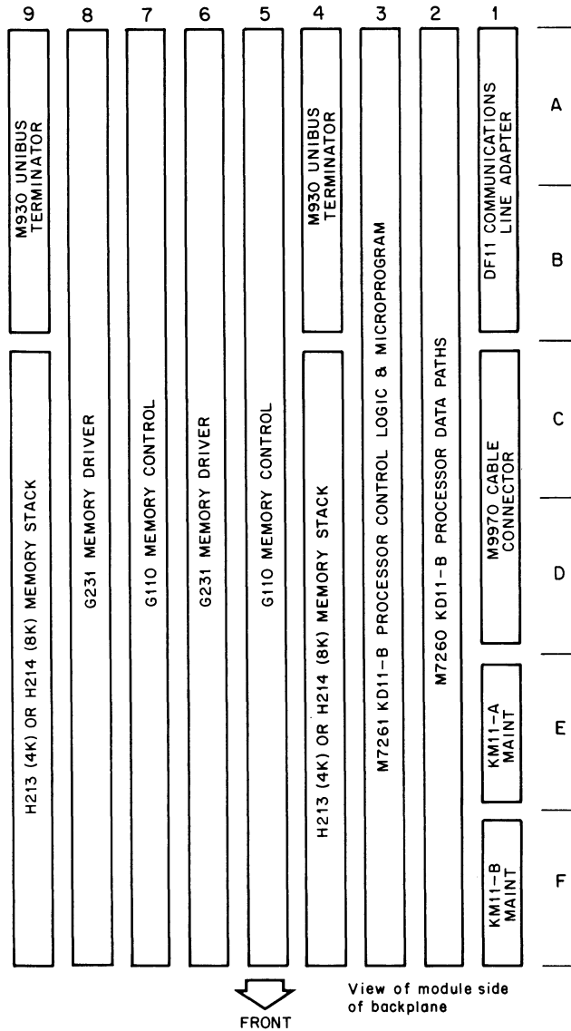
Figure 1-9 Module Utilization Diagram
