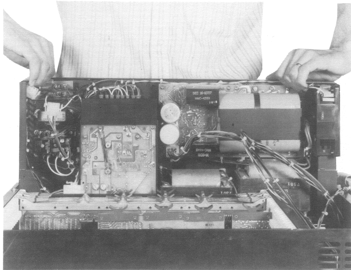
Figure 3-28 Lifting Power Supply From Mounting Box
