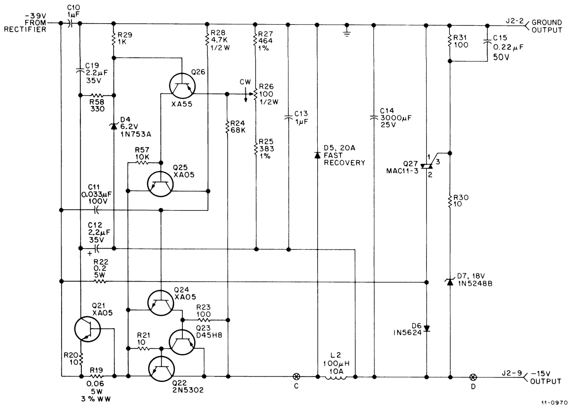
Figure 3-19 -15 V Regulator Circuit
